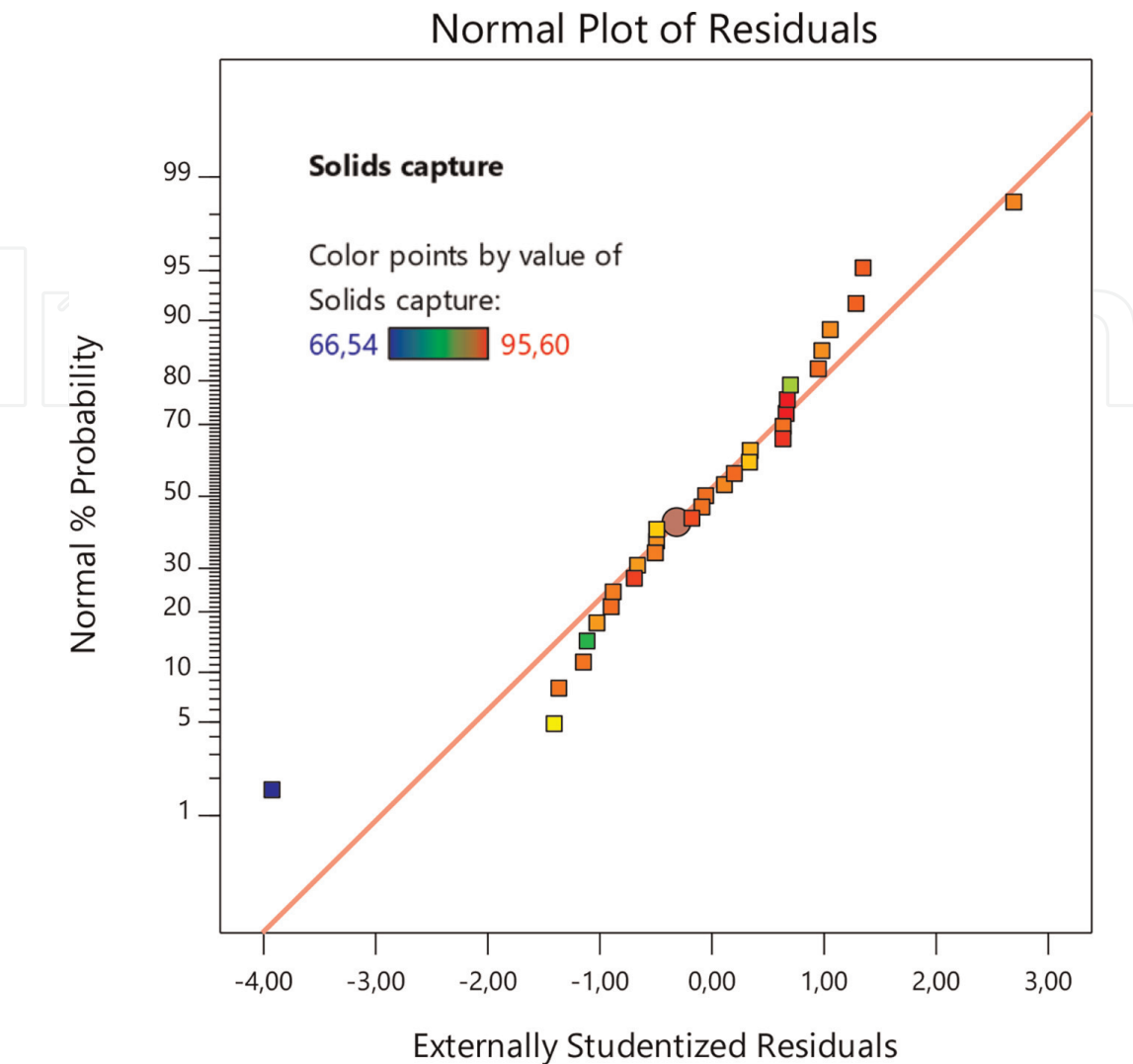
Figure 8. Normal probability plot of residuals for solid capture.
