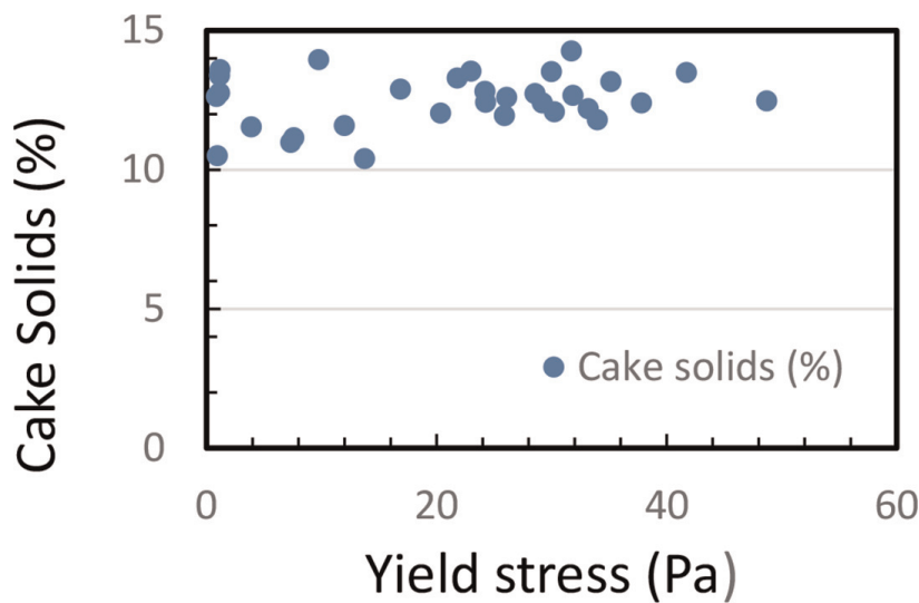
Figure 6. Cake solids as a function of yield stress.
