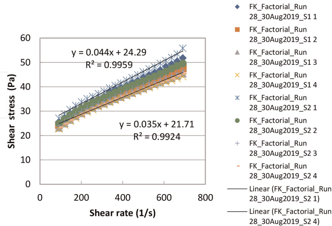
Figure 3. Typical rheogram.
