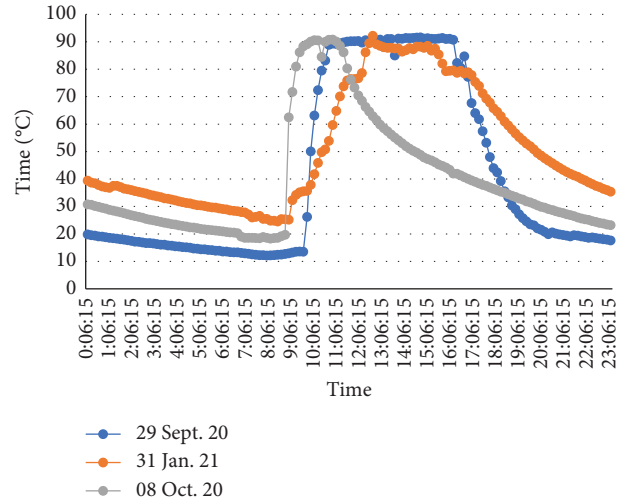
FIGURE 8: Evaporator SW temperature on various days under moderate average solar radiation.
