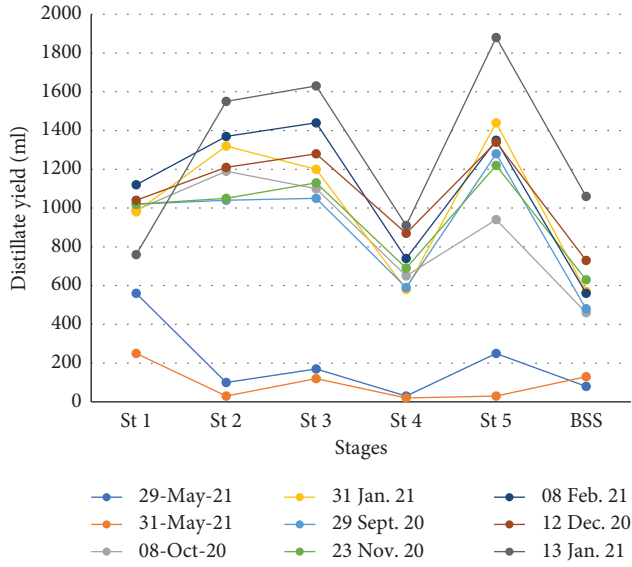
FIGURE 15: Year-round distillate yield trends.
