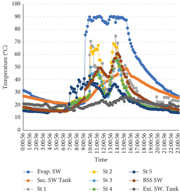
FIGURE 13: SW temperature in the condensing tower under high average conditions (23-Nov-2020).
