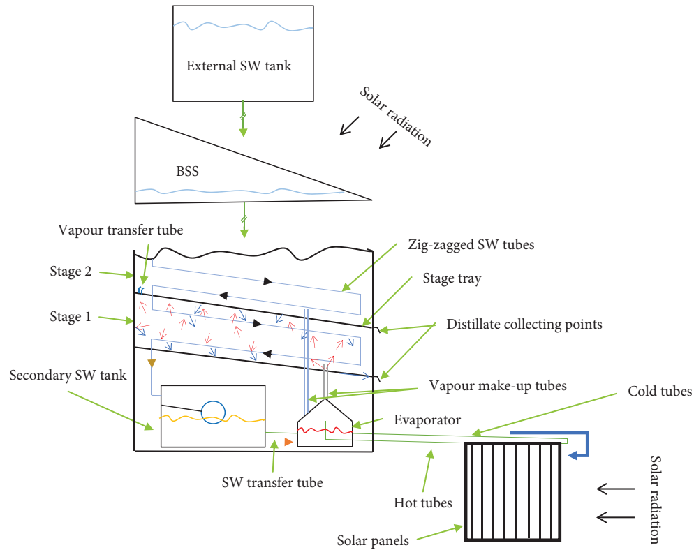
FIGURE 1: MSS-SS schematic diagram.
