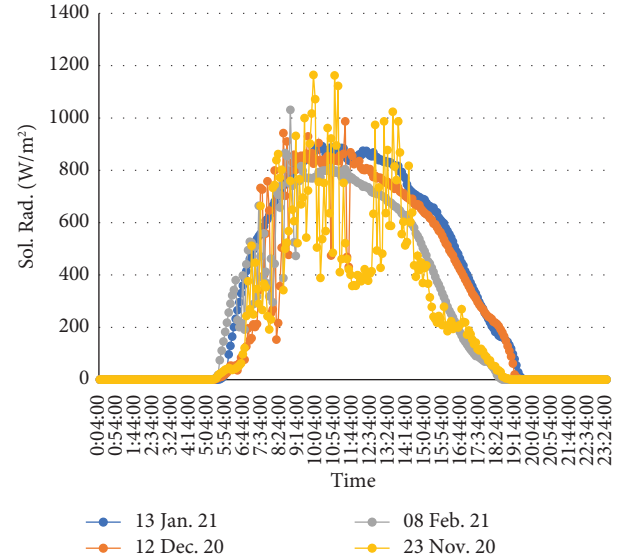
FIGURE 12: Solar radiation curves under high average daily solar radiation.
