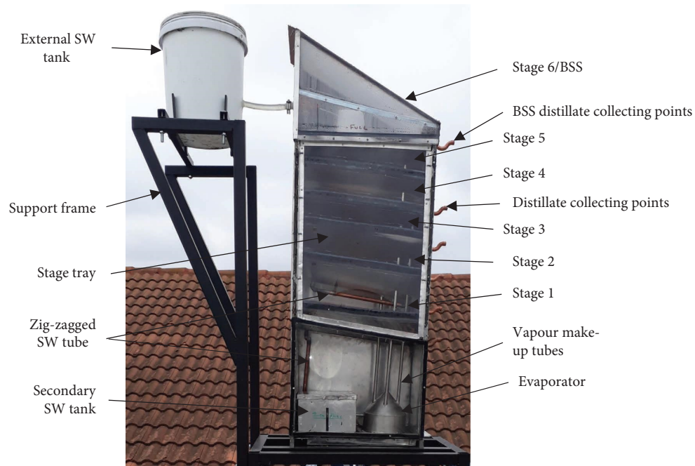
FIGURE 2: Vapour-based MSS-SS.
