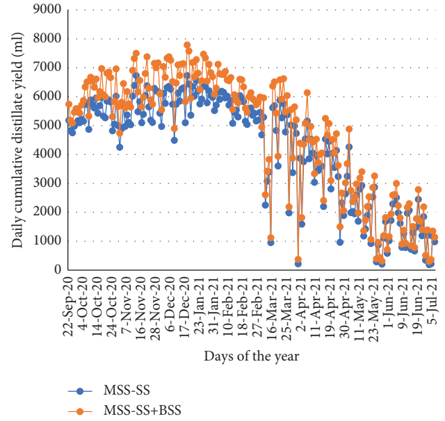
FIGURE 16: Year-round daily cumulative distillate yield trends.
