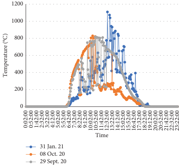
FIGURE 9: Solar radiation curves under moderate average daily solar radiation.
