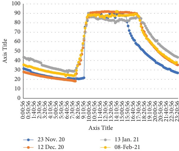
FIGURE 11: Evaporator SW temperature on various days under high average solar radiation.
