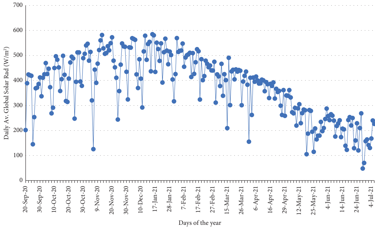
FIGURE 4: Daily average global solar radiation on a horizontal surface.
