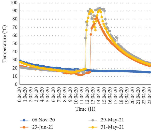
FIGURE 5: Evaporator SW temperature on various days under low average solar radiation.
