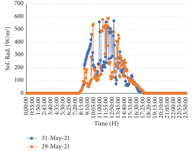
FIGURE 6: Solar radiation curves under low average daily solar radiation.
