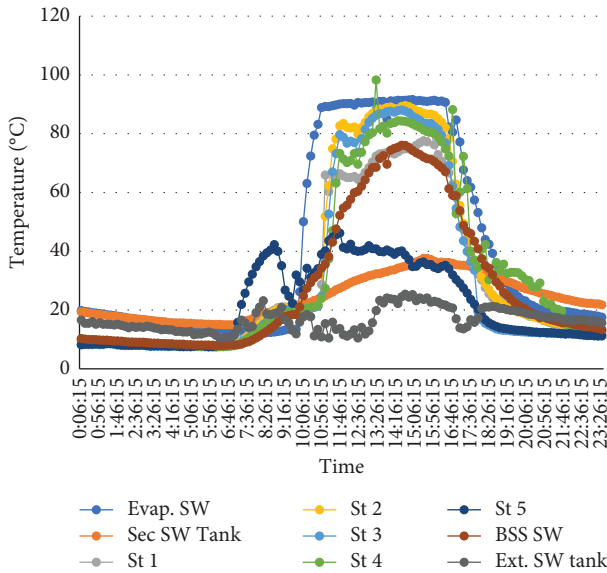
FIGURE 10: SW temperature curves for the 29 th of September 2020.
