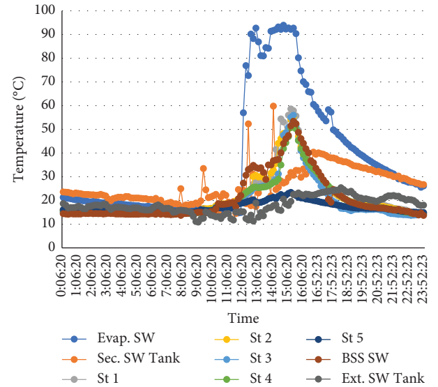
FIGURE 7: SW temperature curves for the 29 th of May 2021.
