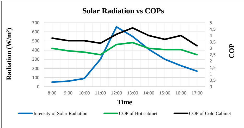
Figure 9. Effect of solar radiation on the COP of both systems
