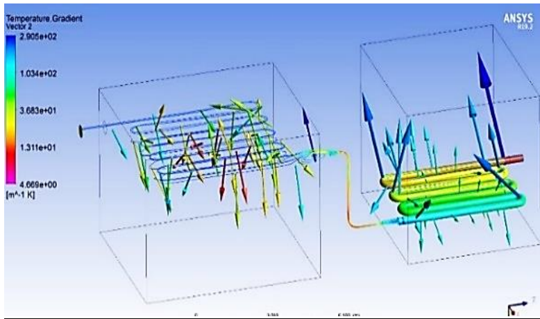
Figure 2. The ISPVRHP simulated air distribution
