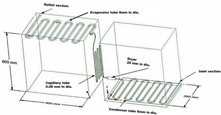
Figure 1. The layout of the evaporator and condenser
