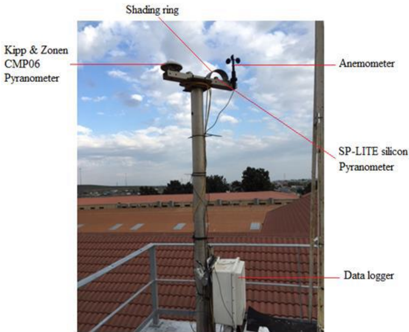
Figure 5. Bellville campus scientific weather station
