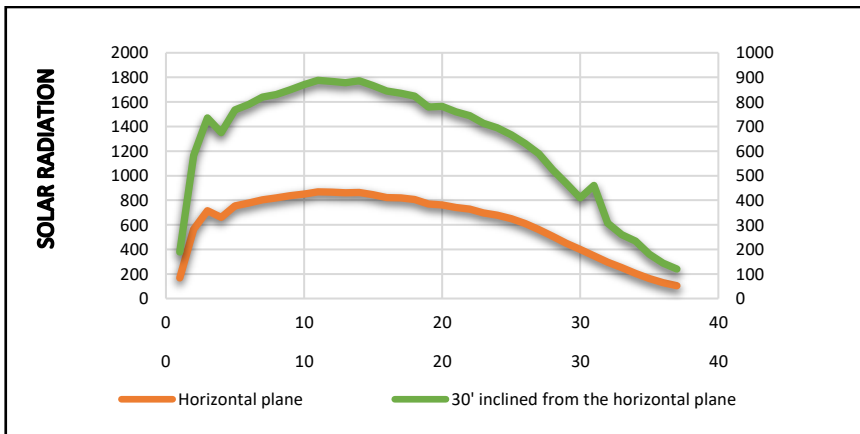
Figure 8. Horizontal PV panels vs 30^\circ tilted PV panels
