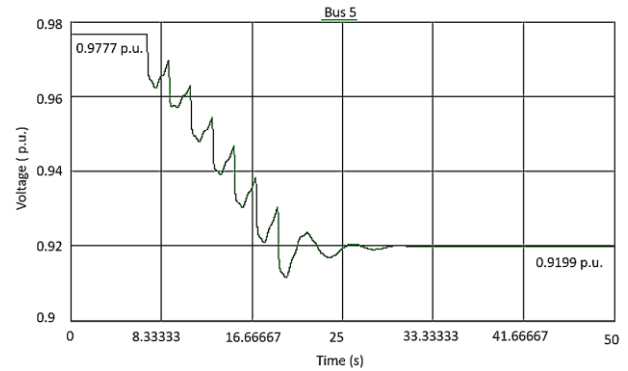
Fig. 3. Impact of 35% load increase on the voltage profile of bus 5
