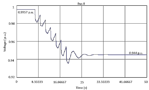
Fig. 4. impact of 35% load increase on voltage profile at bus 8
