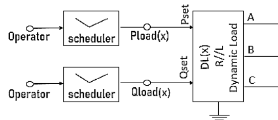
Fig. 2. Control logic for dynamic load control
