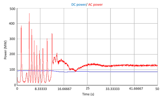
Fig. 10. Non-ideal photovoltaic power dispatch to the grid
