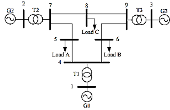
Fig. 1. IEEE-9 bus power system
