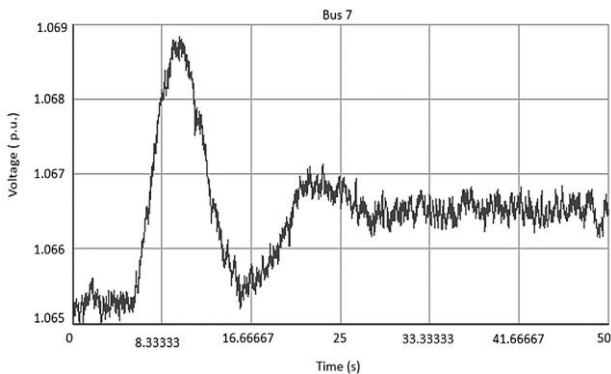
Fig. 9. Influence of non-ideal photovoltaic penetration on bus 7
