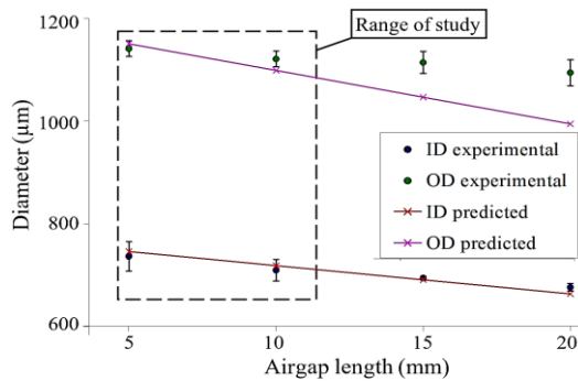
Fig. 10. experimental measurements and predicted values of ID and OD at various AG.
