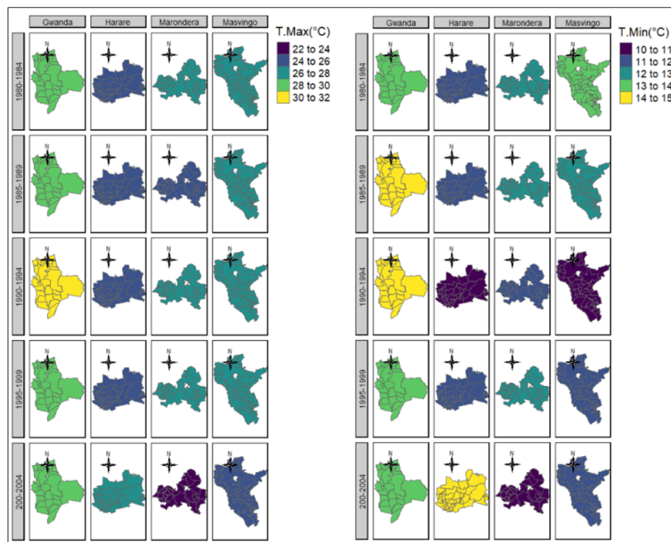
Figure 9. Temperature changes at 5-year intervals in the districts where meteorological stations are located in Zimbabwe.
