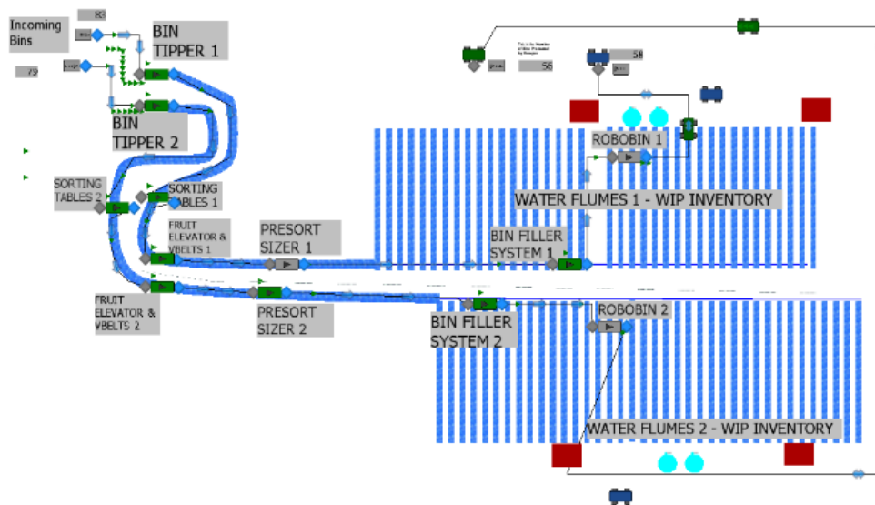
Figure 2: Top view of Design Concept 1
