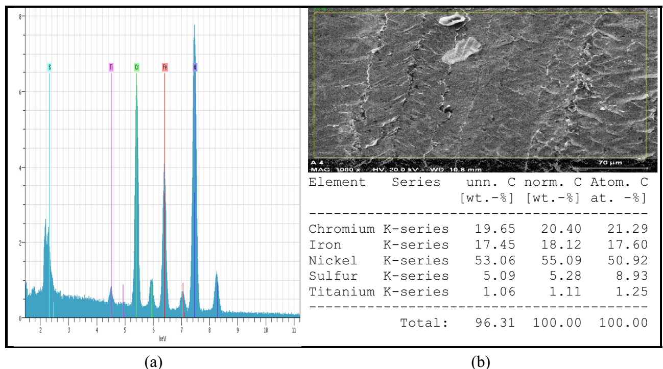
Figure 4. EDS analysis of Inconel 718.
