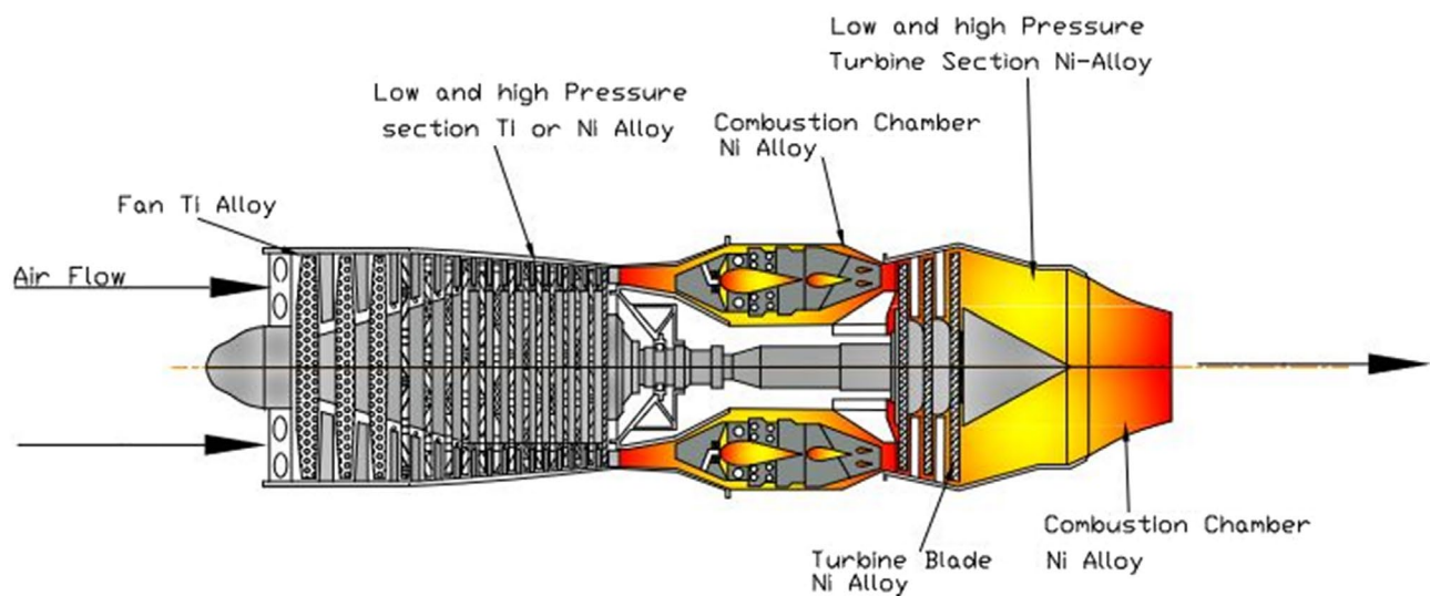
Figure 2. Utilises for nickel-based superalloys, which typically account for around 50% of a jet engine's weight.
