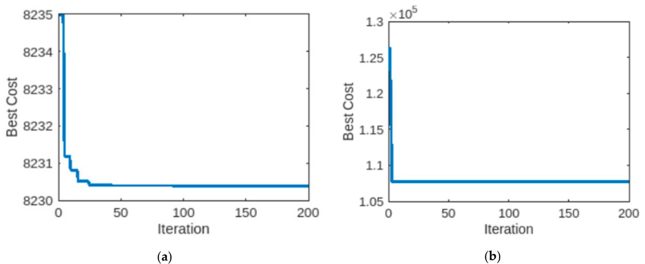
Figure 3. 3-Unit EPD simulation for the minimum cost (best cost): (a) convergence of the minimum cost (best cost) for 3 thermal units, and (b) second-run convergence of the minimum cost (best cost) for 2 thermal and 1 solar PV units.
