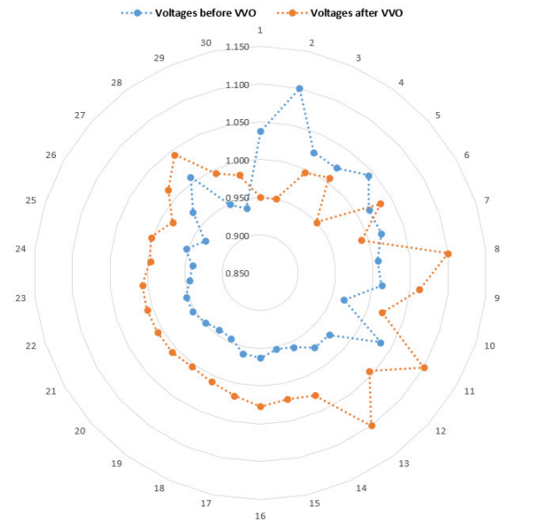
FIGURE 8. Voltage profile of the 30-bus system prior to and following Volt/VAR optimization.
