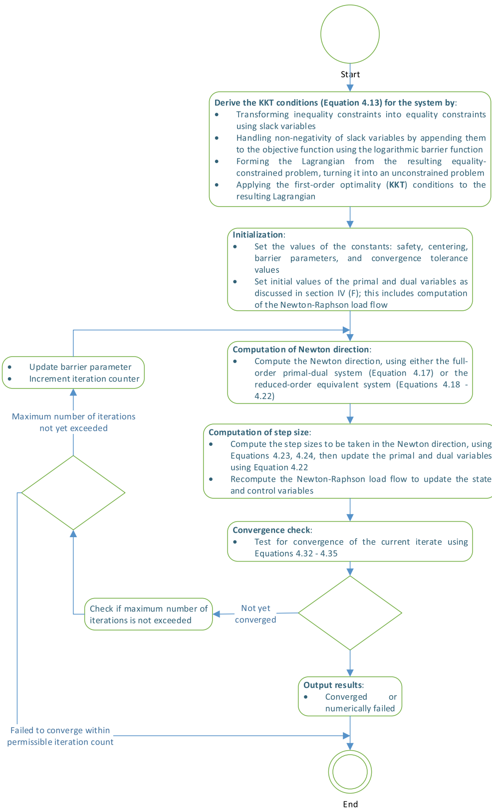
FIGURE 2. Flowchart of the primal-dual interior-point algorithm for VVO.
