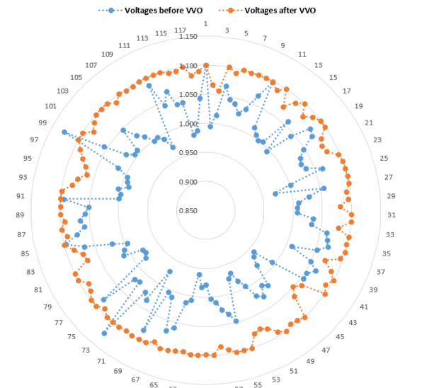
IEEE 118-bus system voltages before and after PSO-based Volt/VAR optimization
