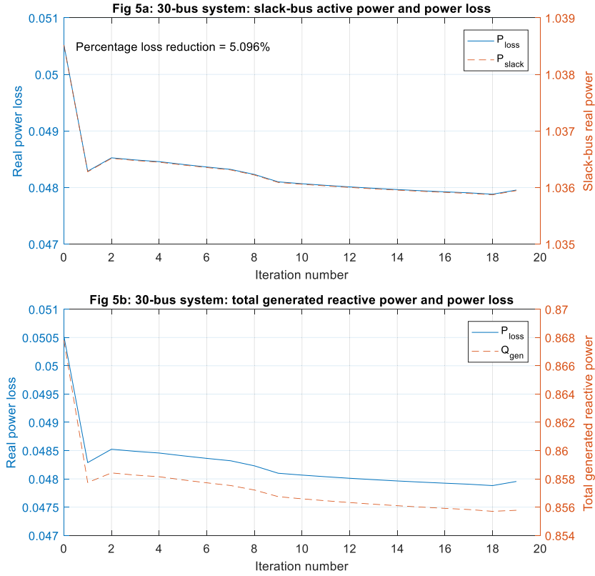
FIGURE 5. 30-bus system comparison of real power loss with slack-bus active power (5a) and with total generated reactive power (5b).
