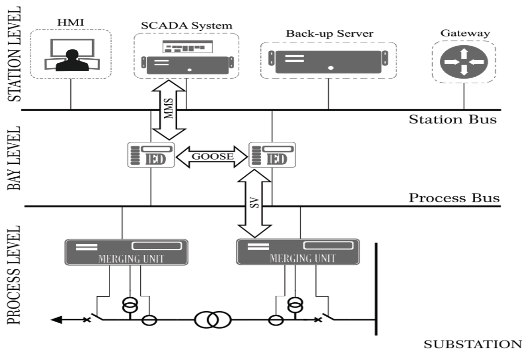
Figure 4. System architecture of IEC61850-based substation [24].
