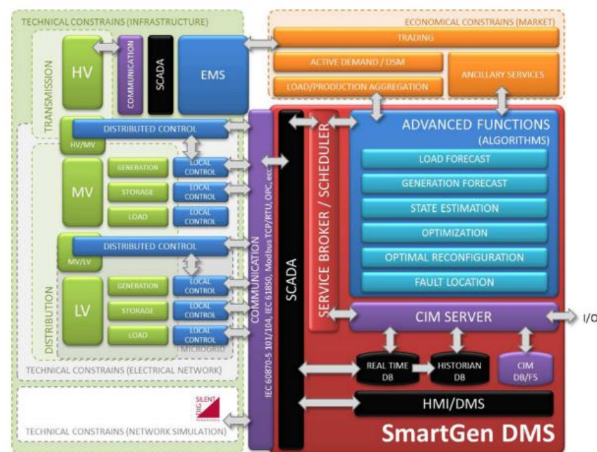
Figure 5. Architecture and key functionalities of a DMS [101].
