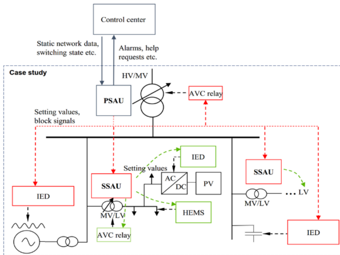
Figure 6. Distributed automation and control architecture [111].
