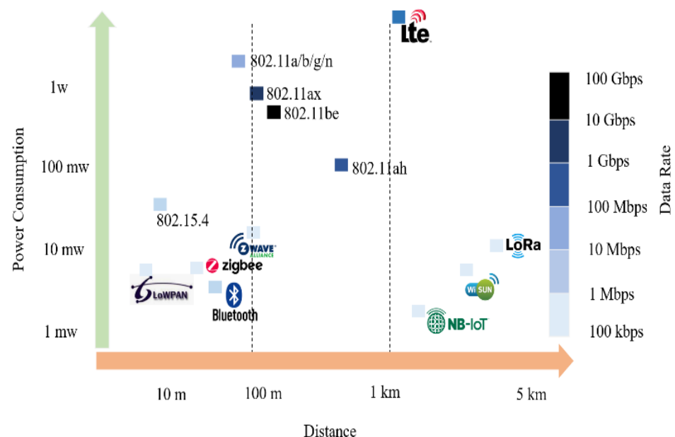
Figure 3. Data rate, coverage distance, and power consumption for various protocols [53].
