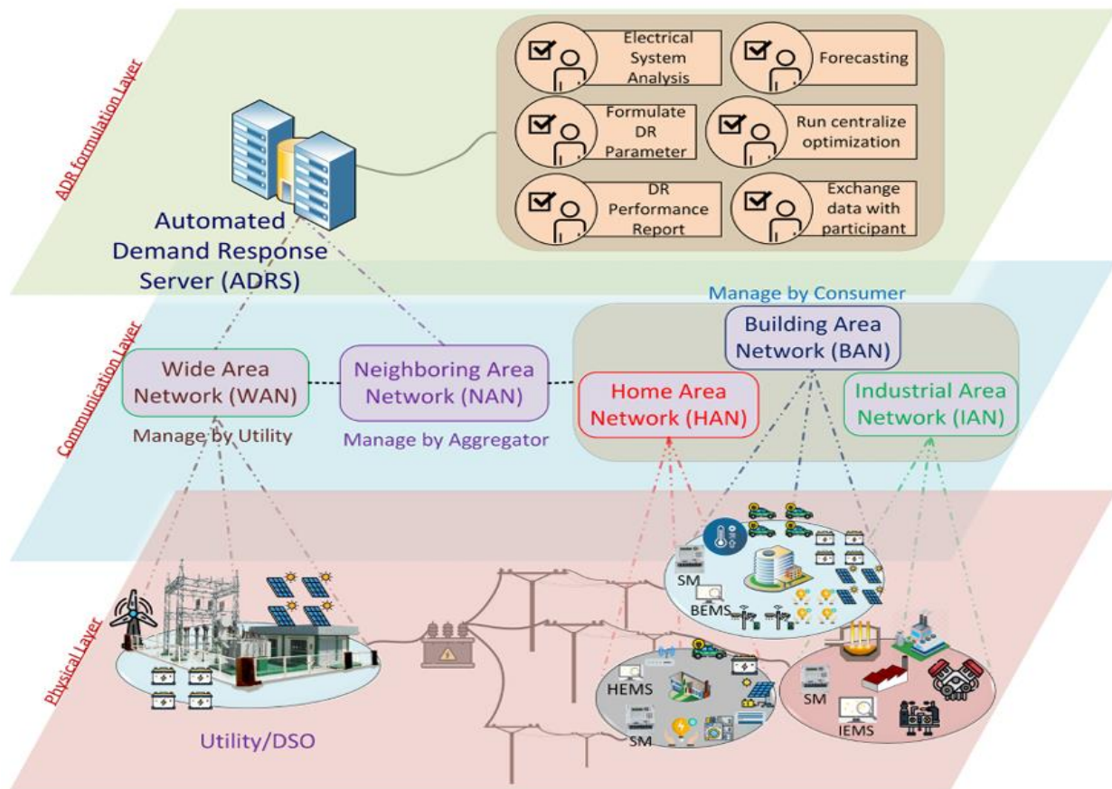
Figure 2. Automated Demand Response Operability layers [32].
