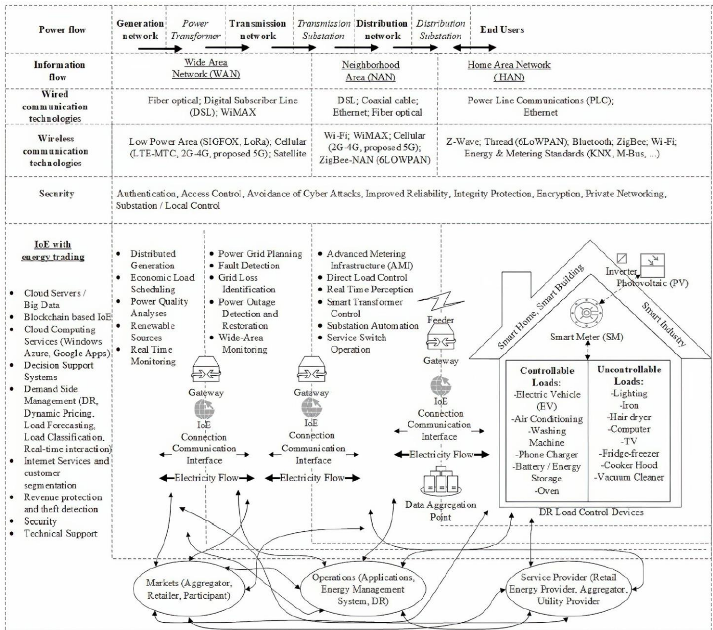
Figure 1. IoE with Energy Components [31].
