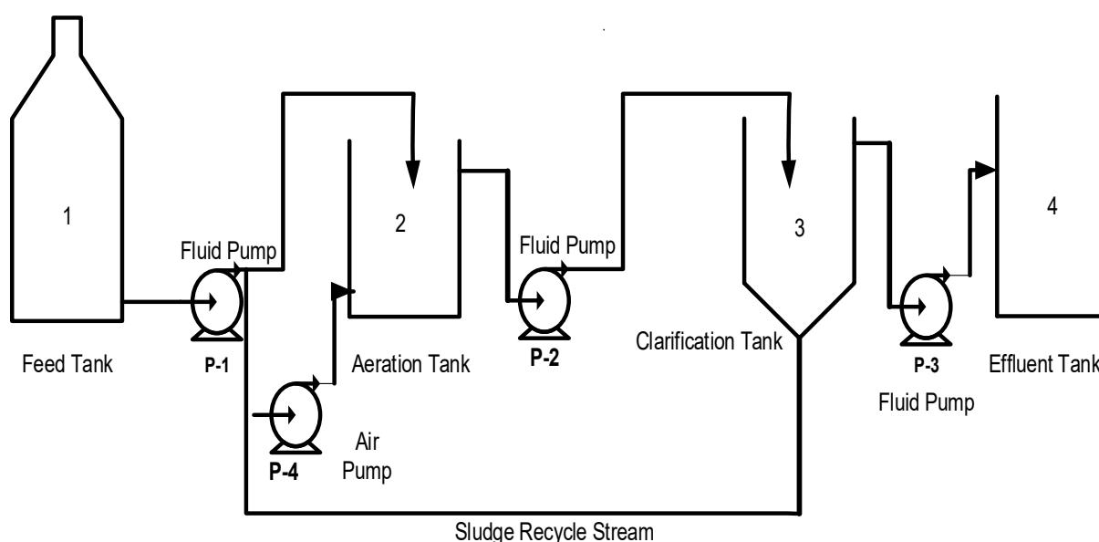
Figure 1. Design of the bench-scale activated sludge treatment system.
