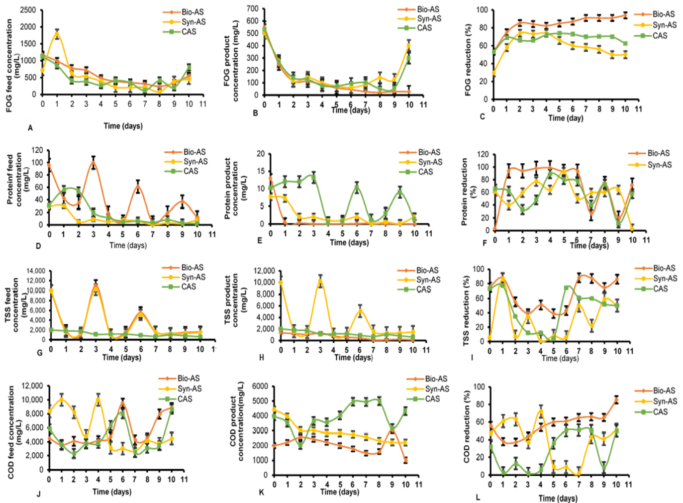
Figure 4. Aeration tank FOG feed (A); aerobic tank FOG product concentration (B); and reduction profiles (C). Protein feed concentration (D); aerobic tank protein product concentration (E); protein concentration reduction profile (F); TSS feed (G); product concentration (H); reduction profile (I); COD feed (J); product concentration (K); and reduction profile (L). All of the above profiles were operated under Bio-AS, Syn-AS, and CAS.
