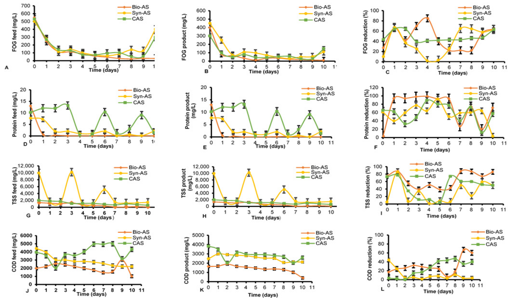
Figure 5. Clarification tank FOG (feed: (A); product concentration: (B), reduction: (C)); protein (feed: (D); concentration product: (E); reduction: (F)); TSS (feed: (G); product: (H); reduction: (I)); COD (feed: (J); product concentration: (K); reduction: (L))—profiles carried out under Bio-AS, Syn-AS, and CAS.
