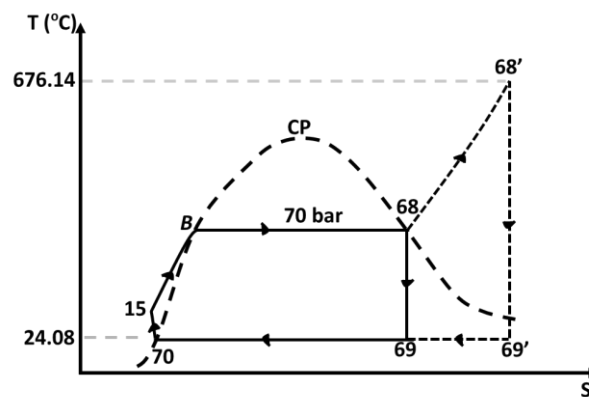
Fig. 3. Temperature versus entropy in the ST system. Line 68-69-70-15-B-68 = saturated cycle. Line 68'-69'-70-15-B-68' = superheated cycle. CP = critical point.
