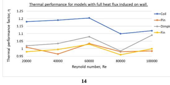
Fig. 9 Thermal performance for model with full heat flux
