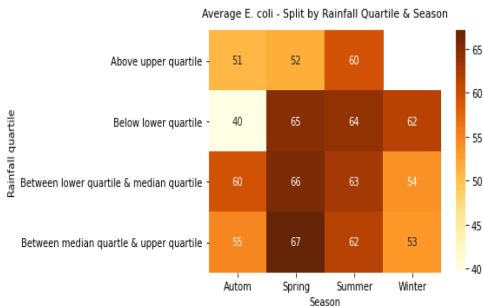
Figure 5. The distribution of Escherichia coli along the Crocodile River from 2016 to 2021 during different seasons.
