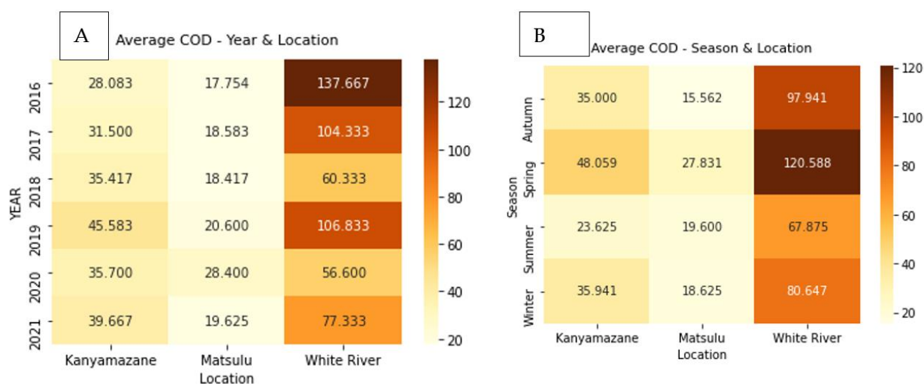
Figure 2. The distribution of COD concentration levels in the sampled sites (White River WWTP, Kanyamazane WWTP, and Matsulu WWTP) in years (A). Spatio-temporal distribution of Chemical Oxygen Demand (COD) seasons in the three sites (B).
