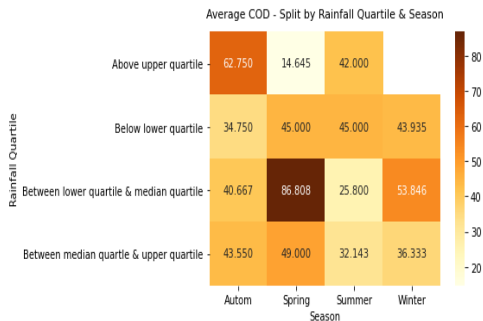
Figure 4. Spatial distribution of COD by seasons with the influence of rainfall. Lower quartile 0.145 mm, Median quartile 0.906 mm, and Upper quartile 2.637 mm.
