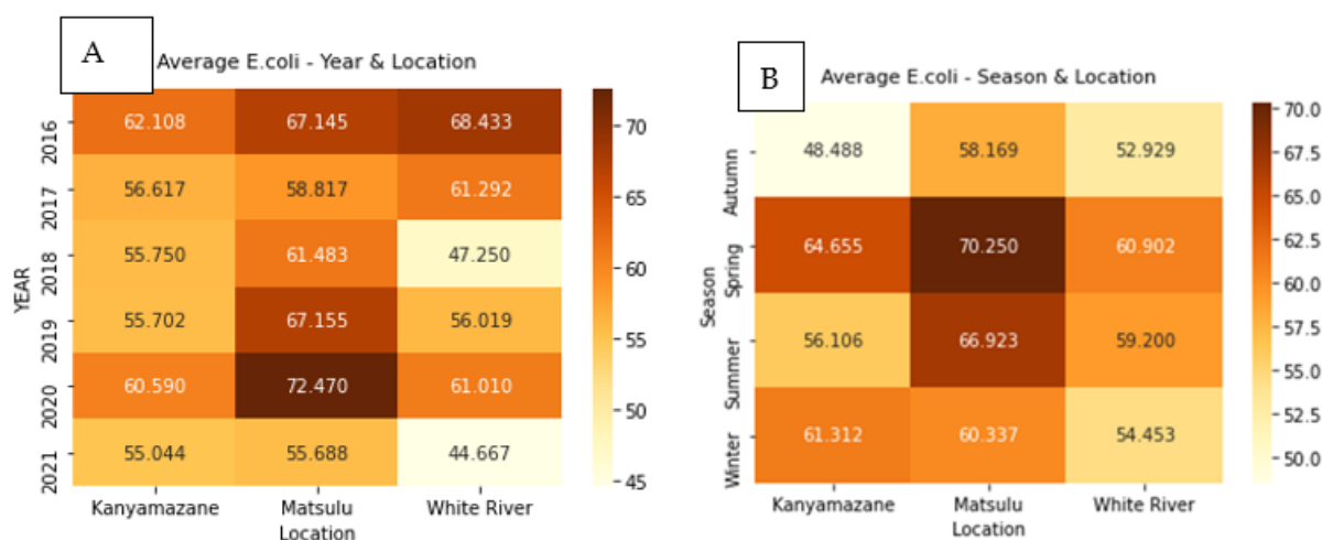
Figure 3. Spatial-temporal distribution of Escherichia coli levels from the three WWTP sampled in the Crocodile River (A). E. coli concentrations at each sampling site for all four seasons (B).
