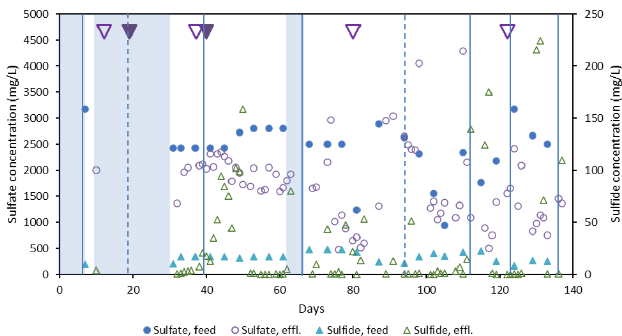
Figure 2. Change in the sulfide and sulfate concentrations over the HLFCR system adapted from [14]. Dashed and full vertical lines indicate biofilm harvest and disruption events, respectively, and shading indicates periods of batch operation. Effl. = effluent.
