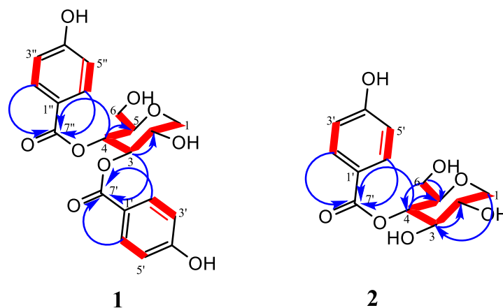
Figure 2. Key HMBC (→) and COSY (→) correlations of compounds 1 and 2 .
