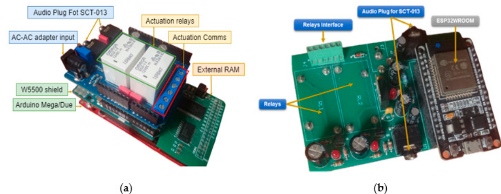
Figure 7. IoTivity HAN servers (appliance interface nodes): (a) AVR/ARM DAQ node prototype; (b) ESP32 node DAQ Prototypes.
