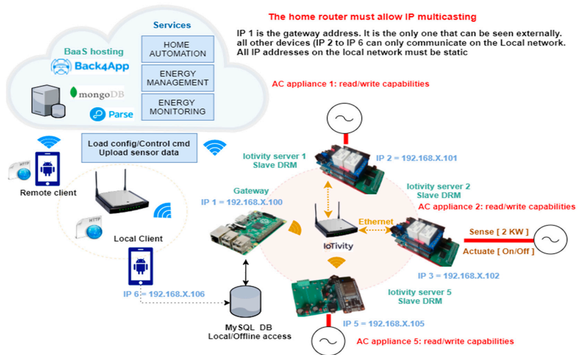
Figure 13. Case study system architecture.
