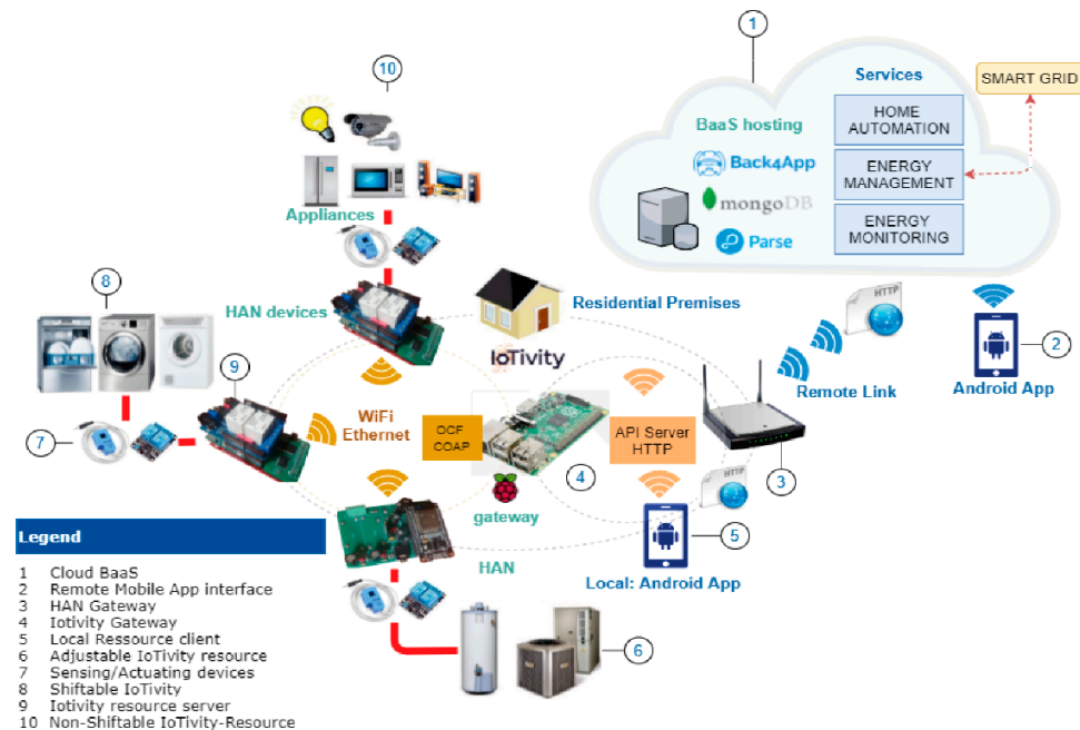
Figure 2. Cloud-based IoTivity-Lite platform HEM architecture.
