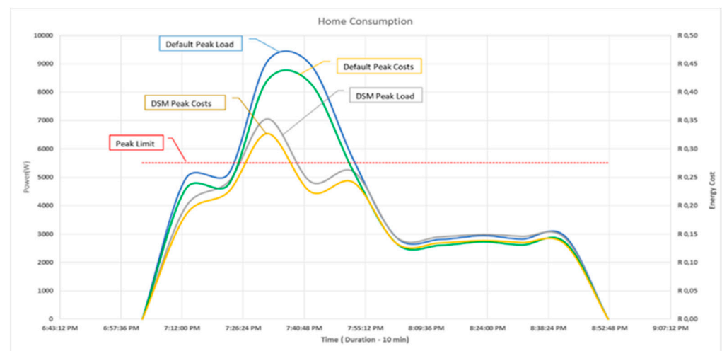
Figure 15. Peak load profiling via IoTivity HEM platform.
