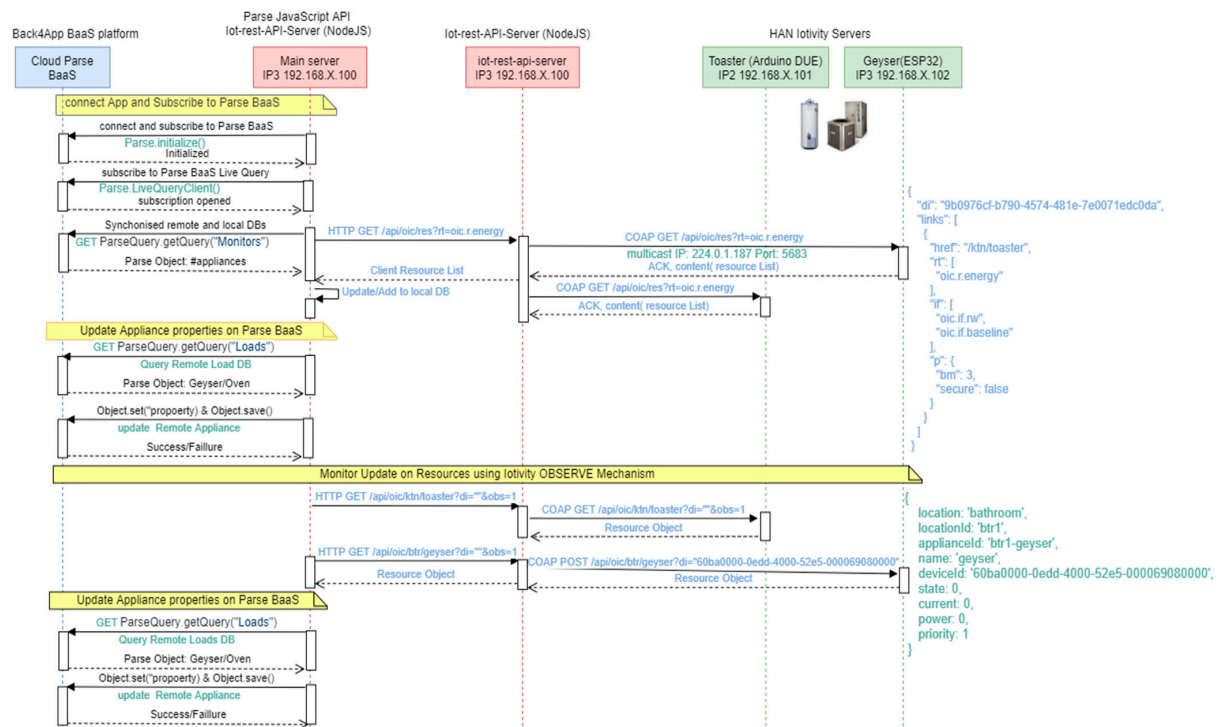
Figure 4. Local and cloud configuration and communication in the platform.
