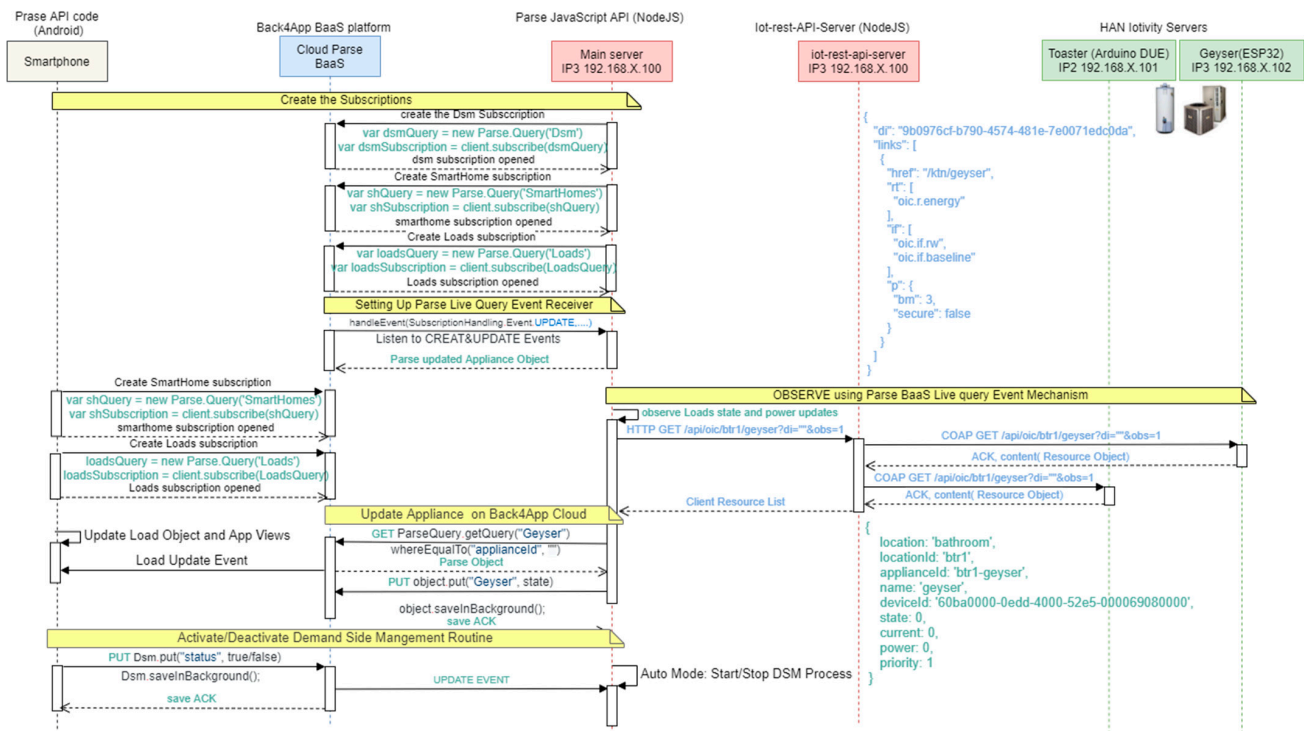
Figure 5. Communication flow with remote/local Android smartphone app.
