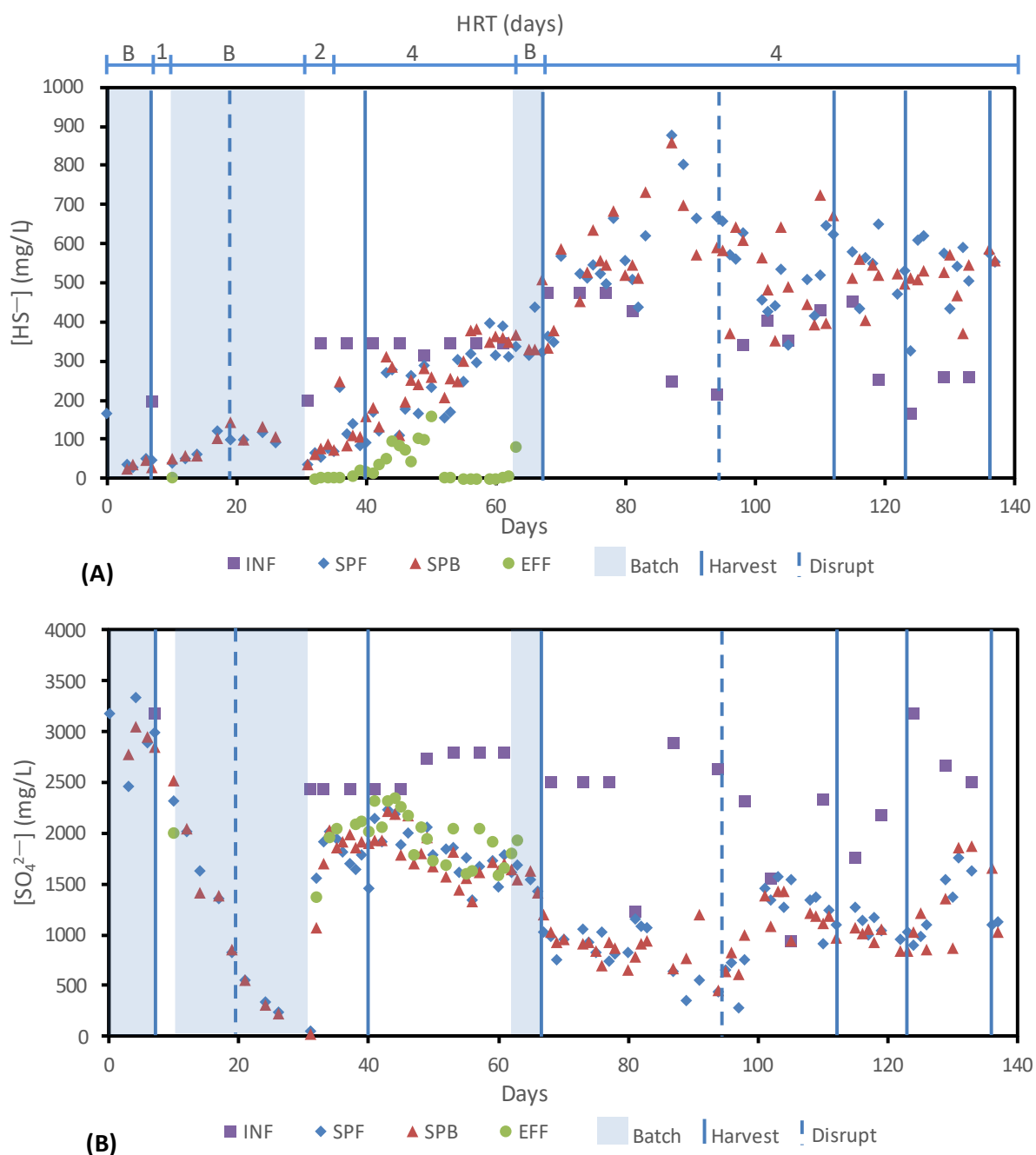
Figure 2. Change in the (A) \text{HS}^- and (B) \text{SO}_4^{2-} concentrations in HLFCR1. Vertical lines and shading indicate biofilm harvest and disruption events and periods of batch operation. INF = influent, SPF = sampling port front, SPB = sampling port back and EFF = effluent.
