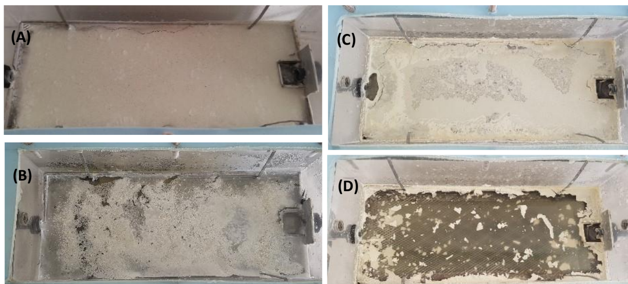
Figure 5. Floating sulfur biofilm formation. (A) HLFCR1, day 2, showing the first biofilm that formed. (B) HLFCR2, day 53, four days after seeding with saline-adapted, dried biofilm. (C) HLFCR1, day 40, prior to harvesting. (D) HLFCR1, day 40 after harvest, showing residual biofilm.
