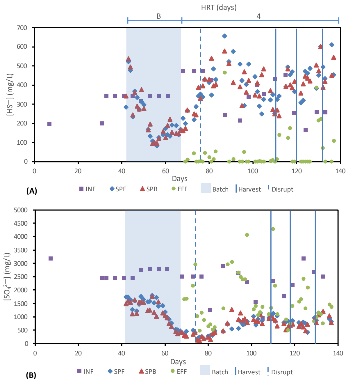
Figure 3. Changes in the (A) \text{HS}^- and (B) \text{SO}_4^{2-} concentrations in HLFCR2. Vertical lines and shading indicate the biofilm harvest and disruption events and periods of batch operation. INF = influent to HLFCR1, SPF = sampling port front, SPB = sampling port back and EFF = effluent.
