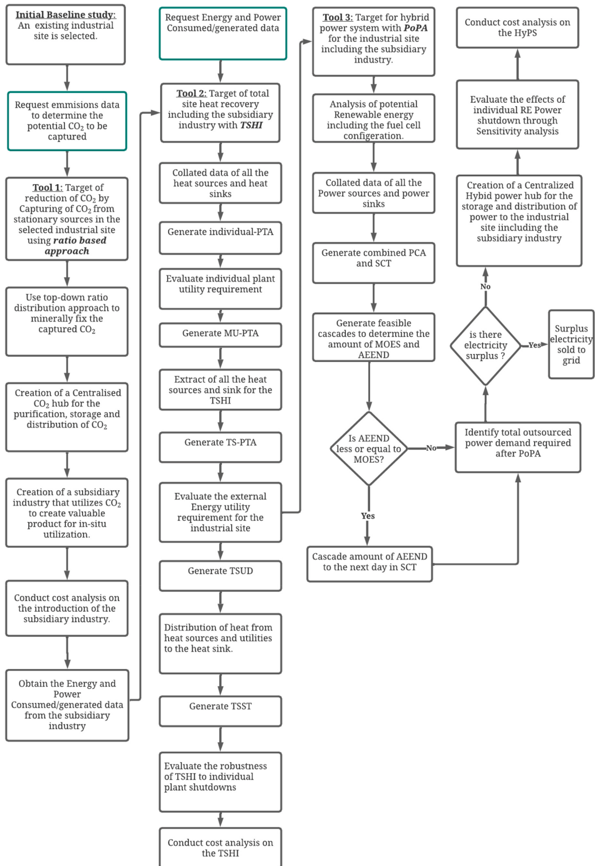
Fig. 2. Sequential procedure to reduce CO 2 of a brownfield industrial site.
