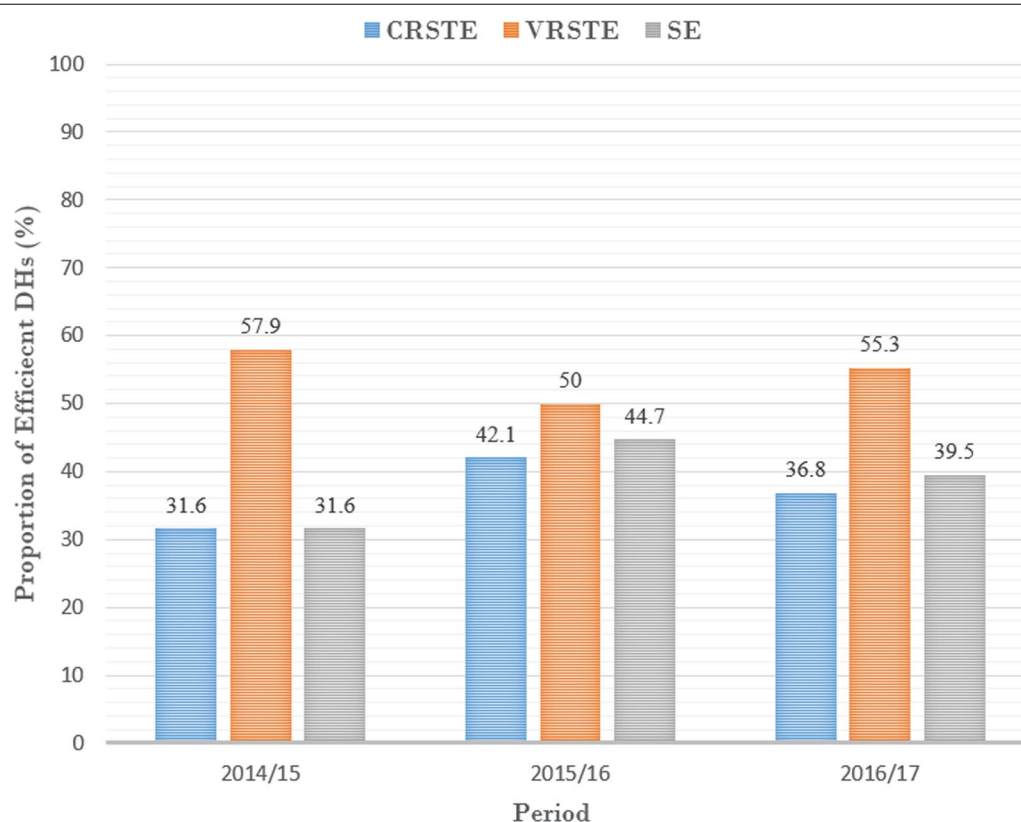
Fig. 1 Distribution of technically efficient district hospitals from 2014/15 to 2016/17
