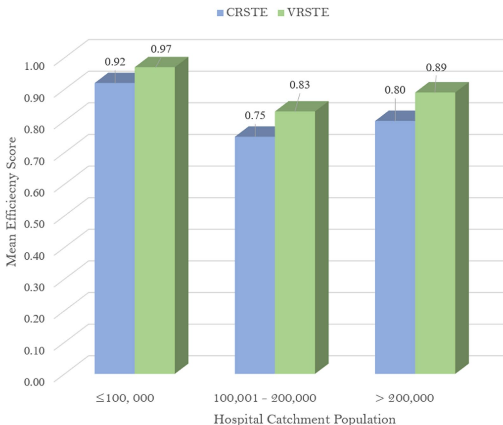
Fig. 2 CRS and VRS technical efficiency based on the catchment population
