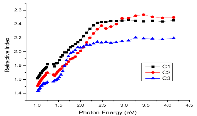
Figure 7. Refractive Index and photon energy of CZFS TFs.
