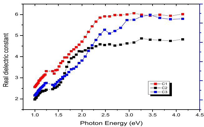
Figure 9. Real dielectric constant and photon energy of CZFS TFs.
