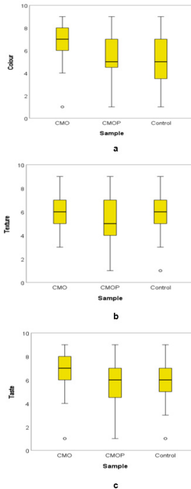
Figure 3. Mean value scores of acceptability: (a) colour, (b) texture and (c) taste scores for CMO (Citric acid + Moringa oleifera leaf extract powder), CMOP (Citric acid + Moringa oleifera leaf extract powder + potassium sorbate) and control dried sliced apples.
