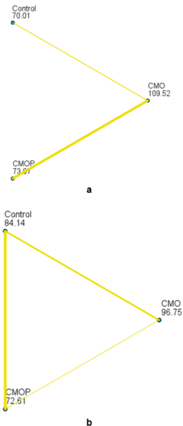
Figure 4. Paired comparison of the samples. Each node shows the sample average rank for (a) colour and (b) texture of the CMO (Citric acid + Moringa oleifera leaf powder), CMOP (Citric acid + Moringa oleifera leaf powder + potassium sorbate) and control dried sliced apples.
