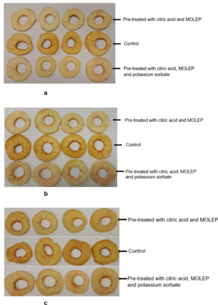
Figure 2. Image of untreated and pre-treated dried apple slices at storage time (a) 0 days; (b) 60 days and (c) 120 days.
