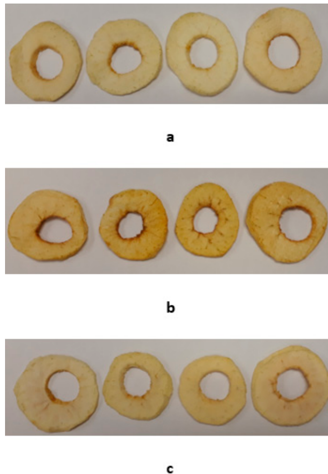
Figure 5. Images of dried apple slices: (a) pre-treated with CMO, (b) control and (c) pre-treated with CMOP at 0 days storage.
