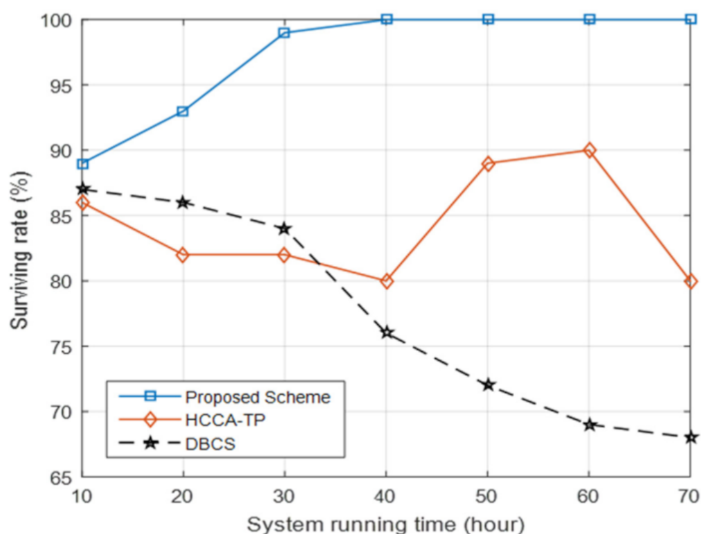
Figure 2. Survival rates of sensor nodes in the network.
