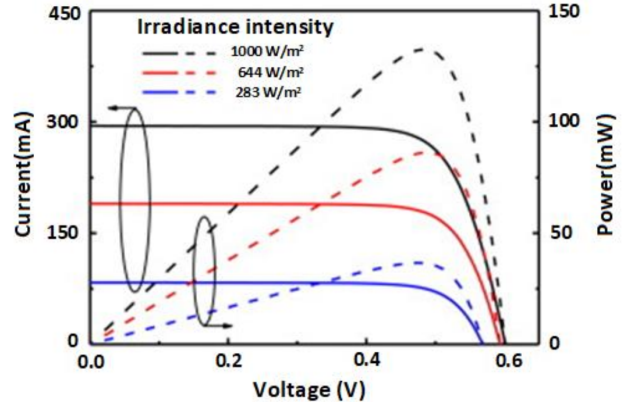
FIGURE 1. The PV cell's characteristics under various solar radiation [24].
