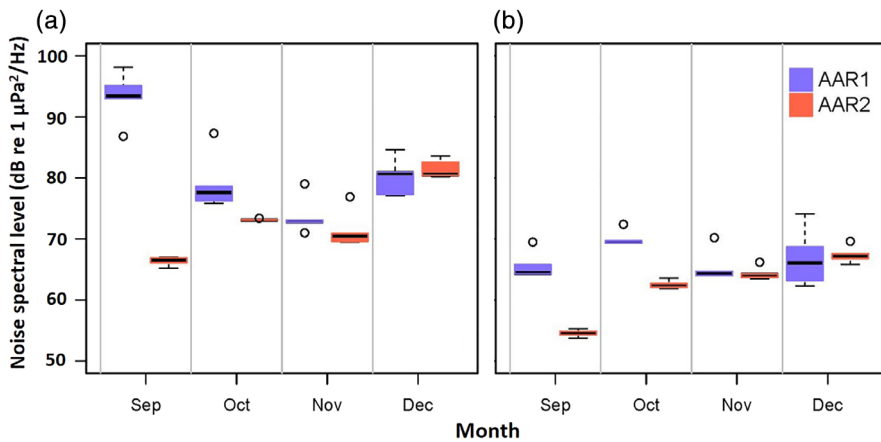
FIGURE 7 Monthly comparison of noise levels at 300 (a) and 2,000 (b) Hz between AARs 1 (purple) and 2 (red). Box and whisker plots are the same as described in the caption of Figure 5, and open circles are observations that are outside the range covered by the whisker.
