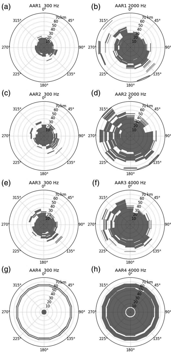
FIGURE 6 Polar plots of BELLHOP model detection range estimates of gunshot sounds for AARs 1 (a, b), 2 (c, d), 3 (e, f), and 4 (g, h) at different bearings (degrees) and frequency bands (300 Hz vs 2,000/4,000 Hz). Gray patches represent regions from which a gunshot sound would be detectable at the hydrophone location (center of plot).
