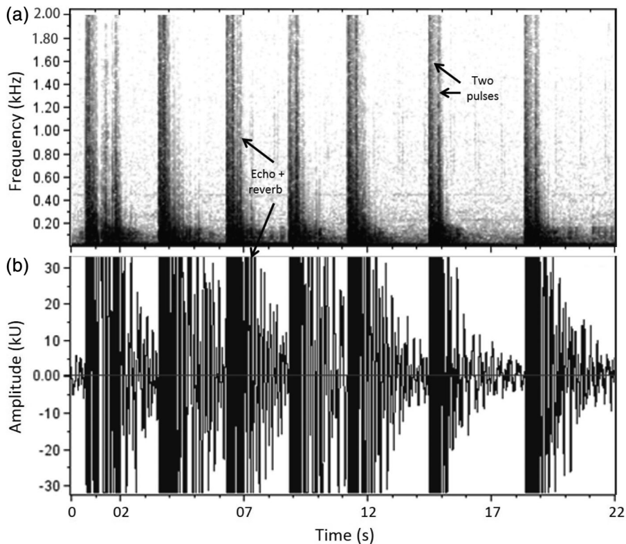
FIGURE 2 Spectrogram of gunshot sounds composed of two pulses together with their echoes and reverberation (a), amplitudes (kU is kilo unit, uncalibrated data) showing clipped waveforms of gunshot sounds (b) recorded by AAR1 on 10 October 2014. Spectrogram parameters: frame size 0.125 s, 50% overlap, FFT size 512 points, Hann window.
