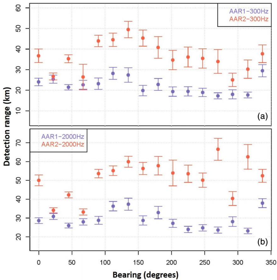
FIGURE 8 Comparison of theoretical maximum detection ranges of AARs 1 and 2 at different bearings. Closed circles represent the mean, and error bars represent the deviations of the data. Median noise levels at 300 Hz from October and September were used for AARs 1 and 2, respectively, and median noise levels at 2,000 Hz from September were used for both AARs (Figure 7).
