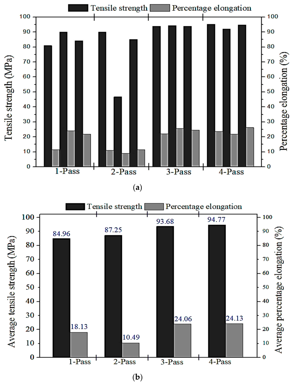
Figure 6. (a) Multiple pass SFSP tensile strength and percentage elongation, (b) average multiple pass SFSP tensile strength and percentage elongation.
