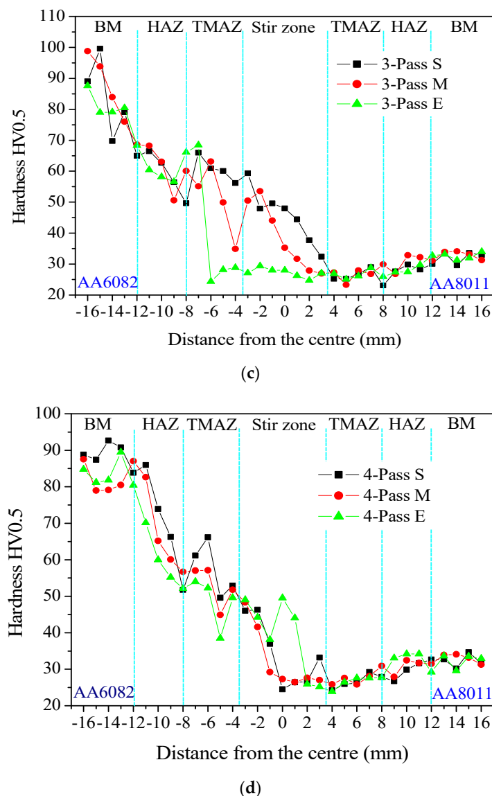
Figure 8. SFSP Hardness profiles, (a) 1-pass, (b) 2-pass, (c) 3-pass and (d) 4-pass.
