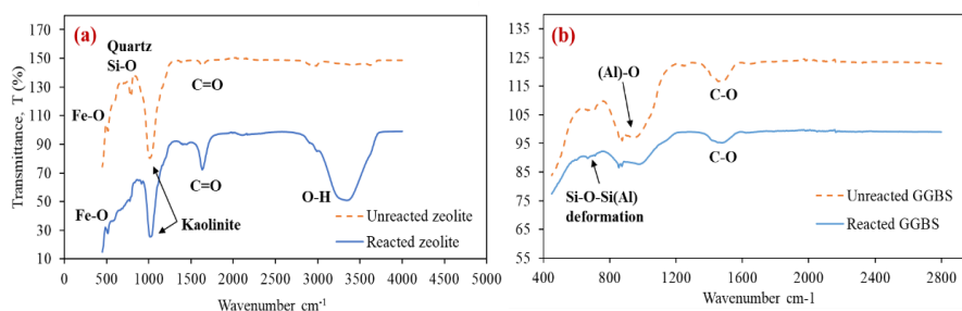
Figure 10. FTIR spectra of (a) zeolite before and after reaction, (b) ground granulated blast-furnace slag (GGBS) before and after reaction with acid mine drainage.
