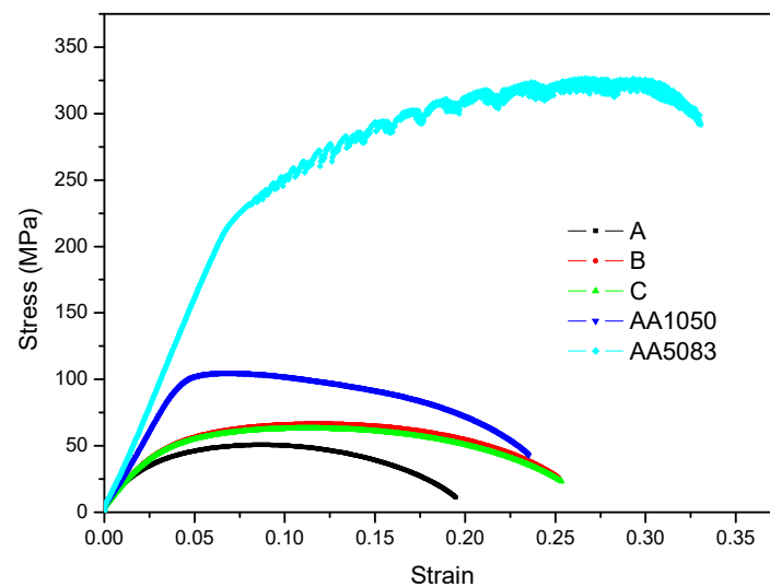
Figure 11. Stress-strain curve.
