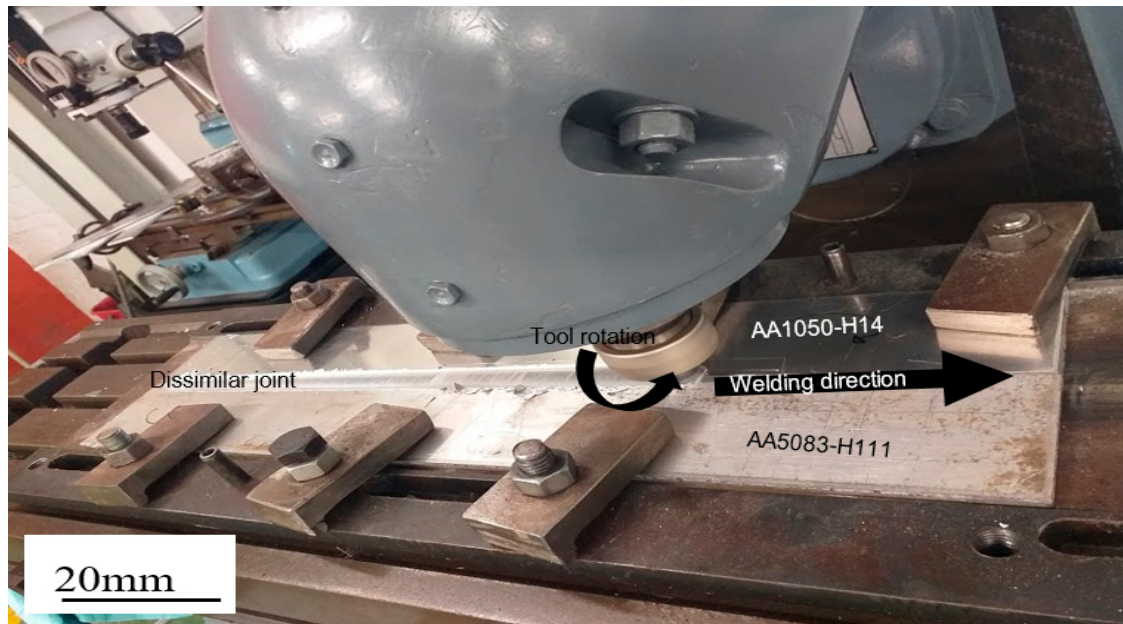
Figure 2. Friction stir welding machine.
