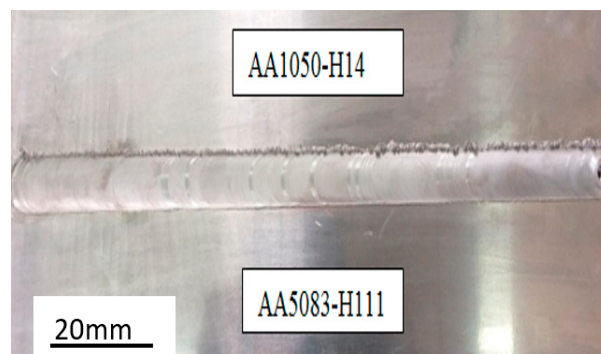
Figure 5. FSW joint.
