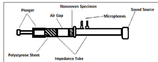
Figure 1. Test setup with a variable air gap between non-woven specimen and polystyrene sheet.
