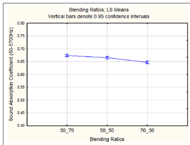
Figure 5. Least square mean values of sound absorption versus blending ratio for all the fabrics.
