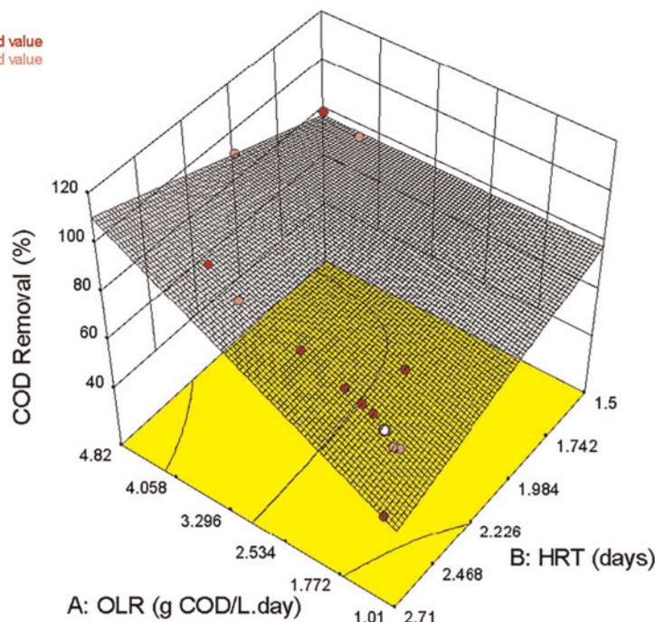
Q8 Figure 2 | 3D plot of OLR (A) and HRT (B), and their effect on EGSB's COD removal efficiency.
