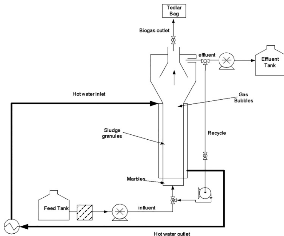
Q7 Figure 1 | Schematic illustration of the EGSB set-up treating PSW.
