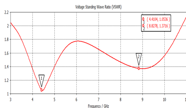
Fig. 4 VSWR characteristics
