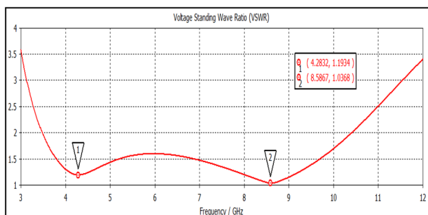
Fig. 7 VSWR characteristics
