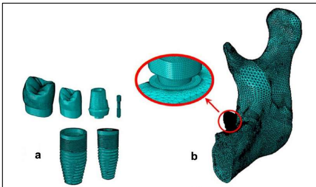
Figure 6. Mesh using linear tetrahedron elements of: (a) the parts of the implant system and (b) the mandibular bone and the final model.
