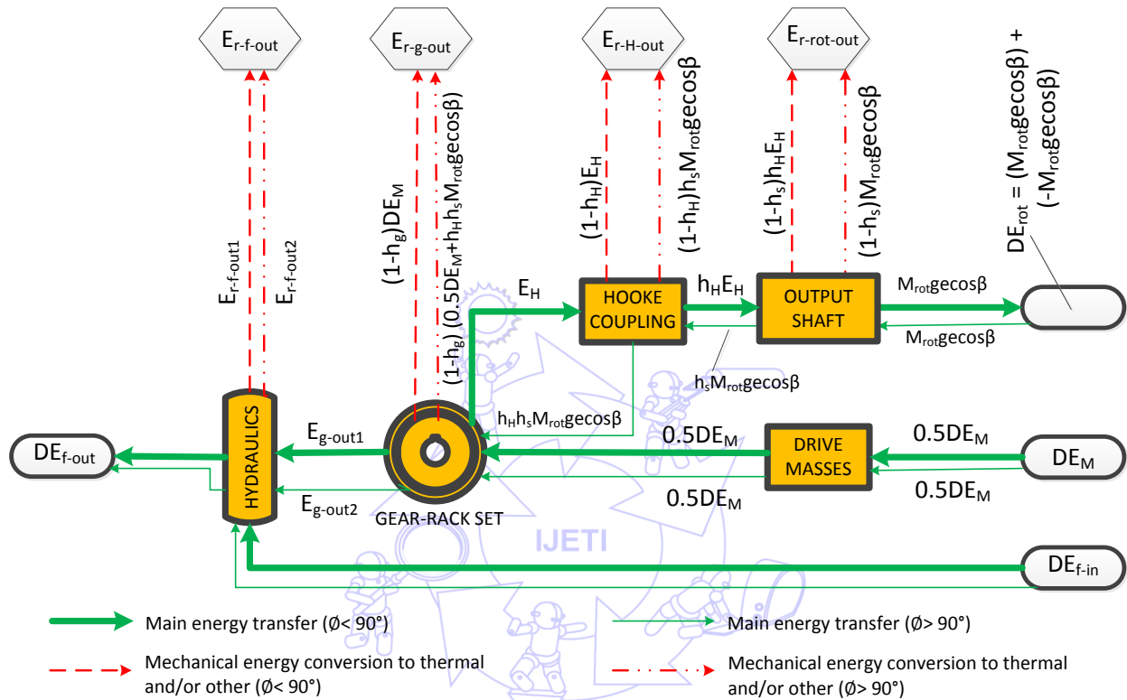
Fig. 5 Energy transfers in the new hydro-mechanism during bladder outflow
