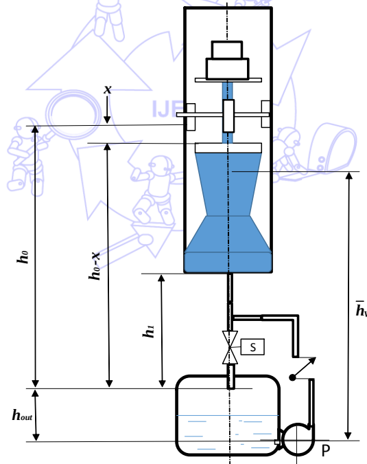
Fig. 3 Fluid flow system
