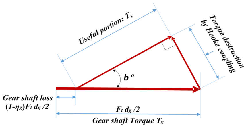
Fig. 2 The gear torque split diagram
