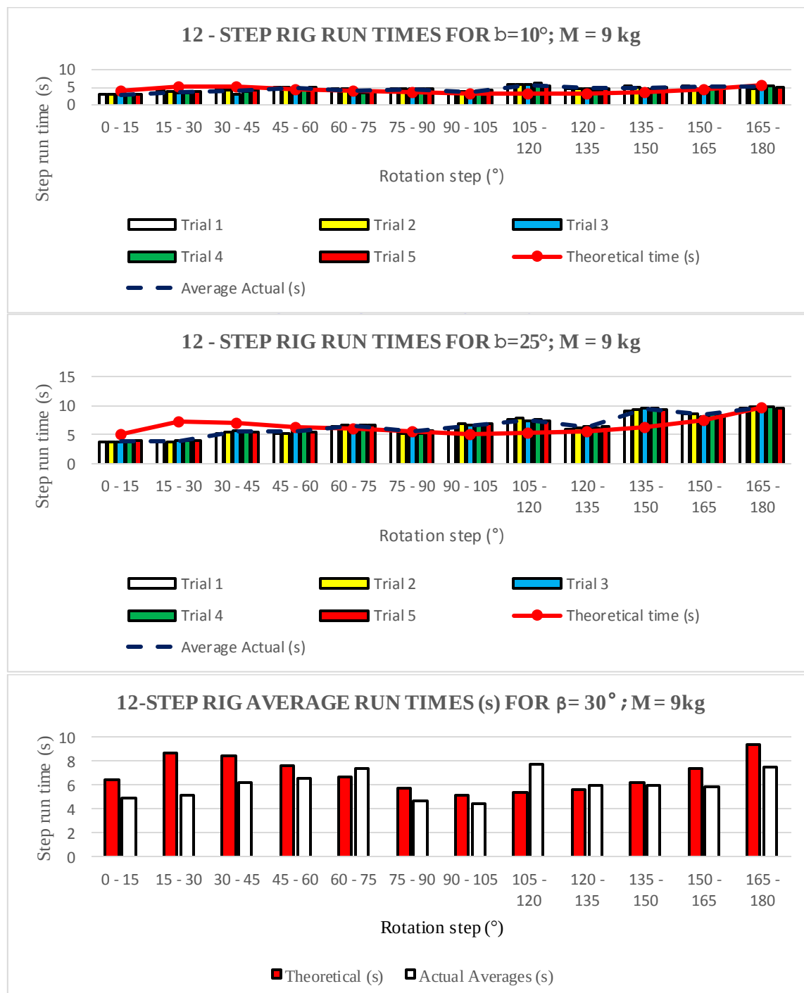
Fig. 8 Verifying efficiencies: theoretical compared with actual run times for \beta = 0^\circ , 25^\circ and 30^\circ
