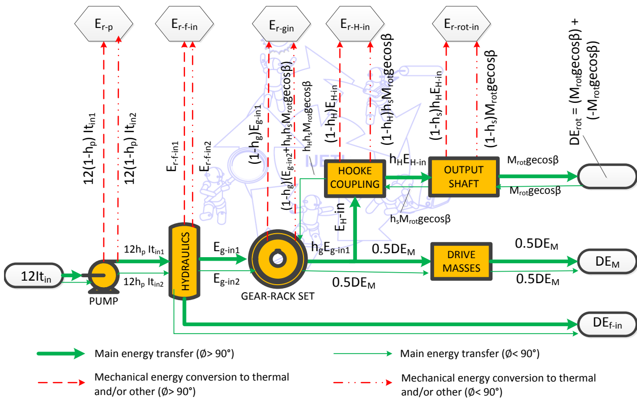
Fig. 4 Energy transfers in the new hydro-mechanism during bladder inflow
