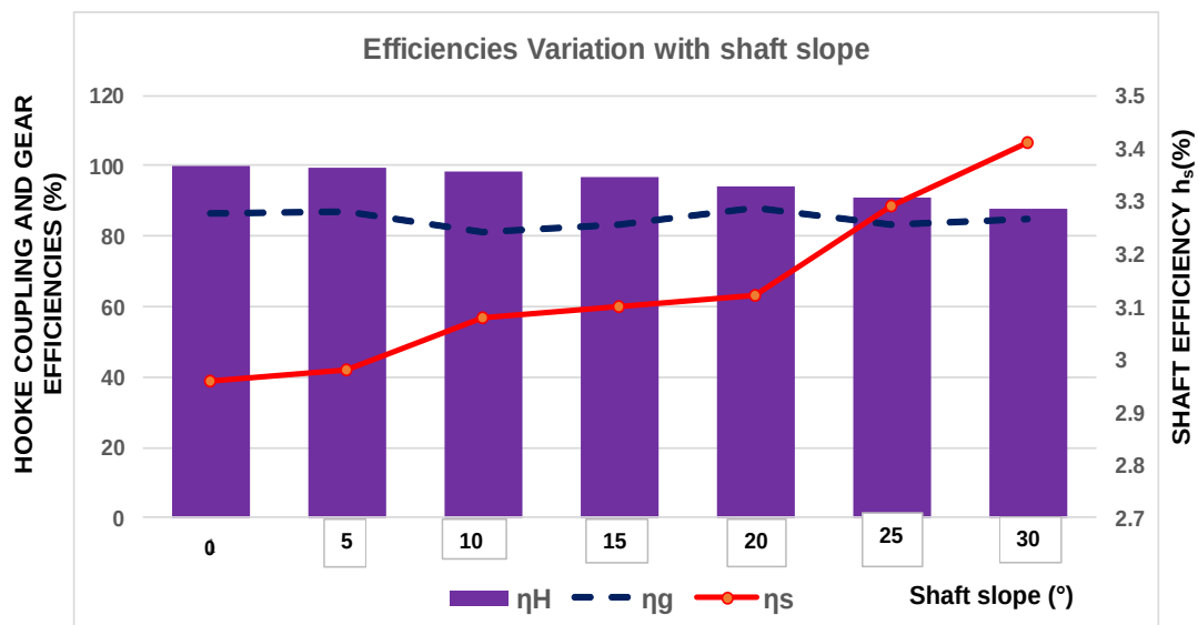
Fig. 7 Variation of mechanical efficiencies with Hooke joint shaft angle
