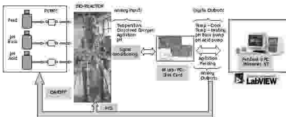
Fig. 1. Hardware Layout
