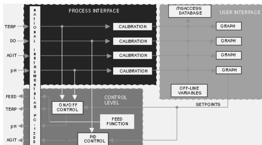
Fig. 2. Software Layout
