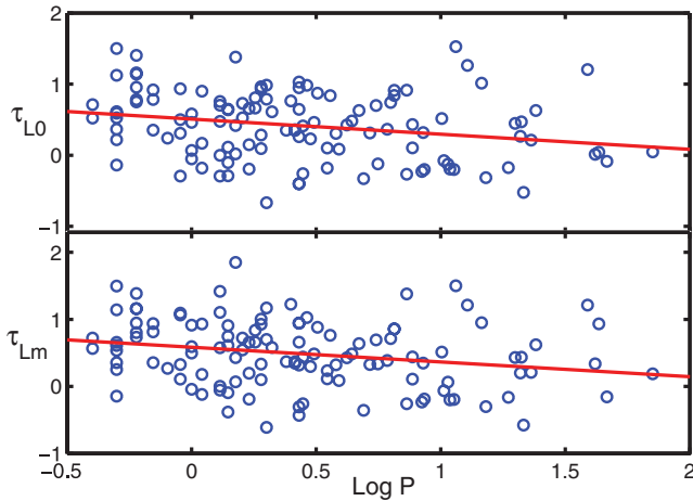
Figure 10. The dependence of ACF widths on the peak flux P : a probable selection effect.
