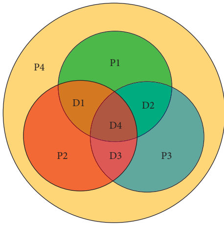
FIGURE 7: Parity relationship to data, extended Hamming (8, 4).
