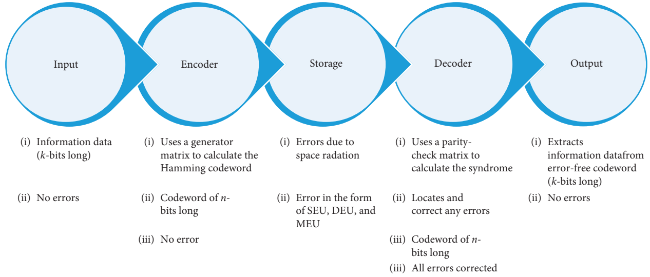
FIGURE 3: General layout of Hamming code.
