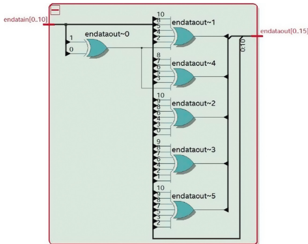
FIGURE 11: RTL overview of the encoder for Hamming [16, 11, 4]_2 .
