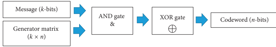
FIGURE 5: Gate/graphical expression of hamming encoder formula.
