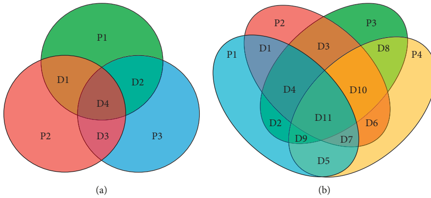
FIGURE 4: Parity vs data: Hamming (7, 3) (a) and Hamming (15, 11) (b).
