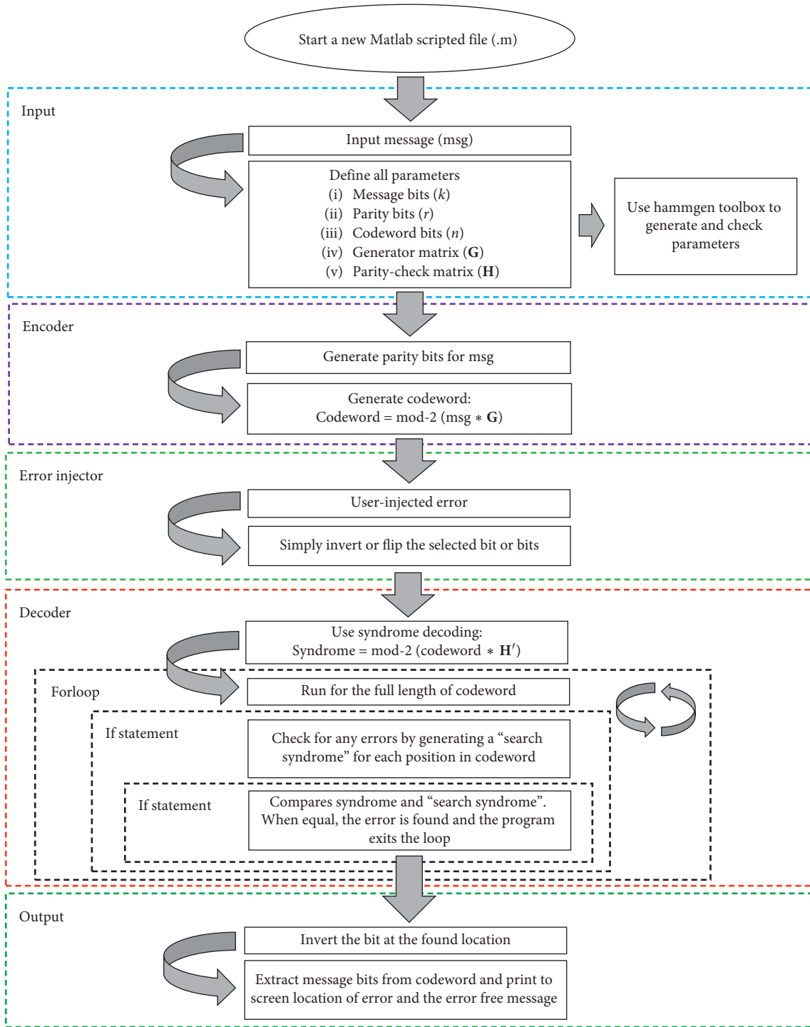
FIGURE 8: Overview of Matlab code (flow chart).
