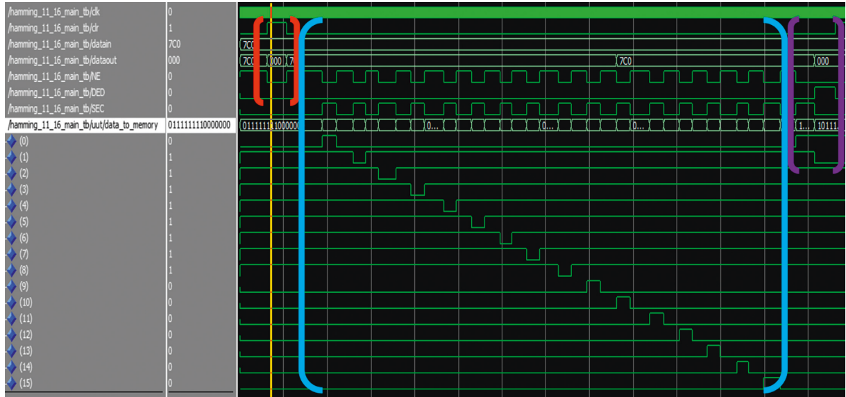
FIGURE 16: ModelSim simulation of Hamming [16, 11, 4] SECDED capabilities.
