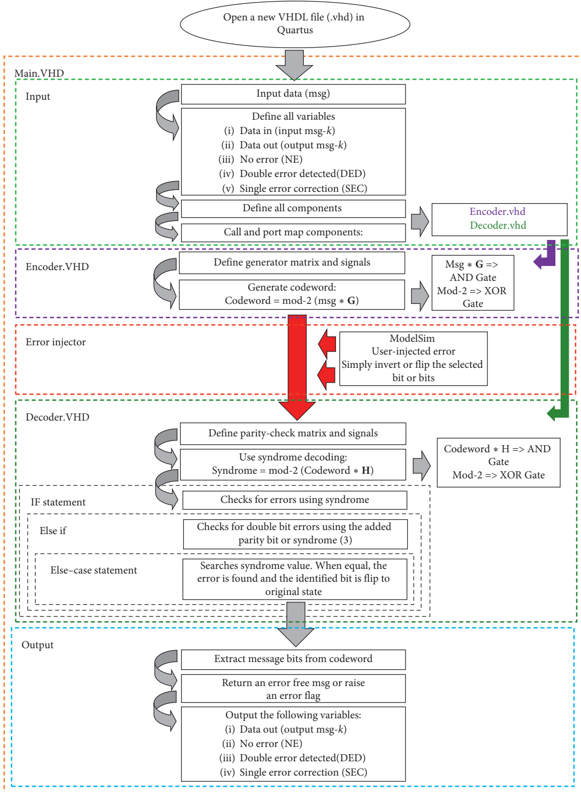
FIGURE 9: Overview of VHDL code (flow chart).
