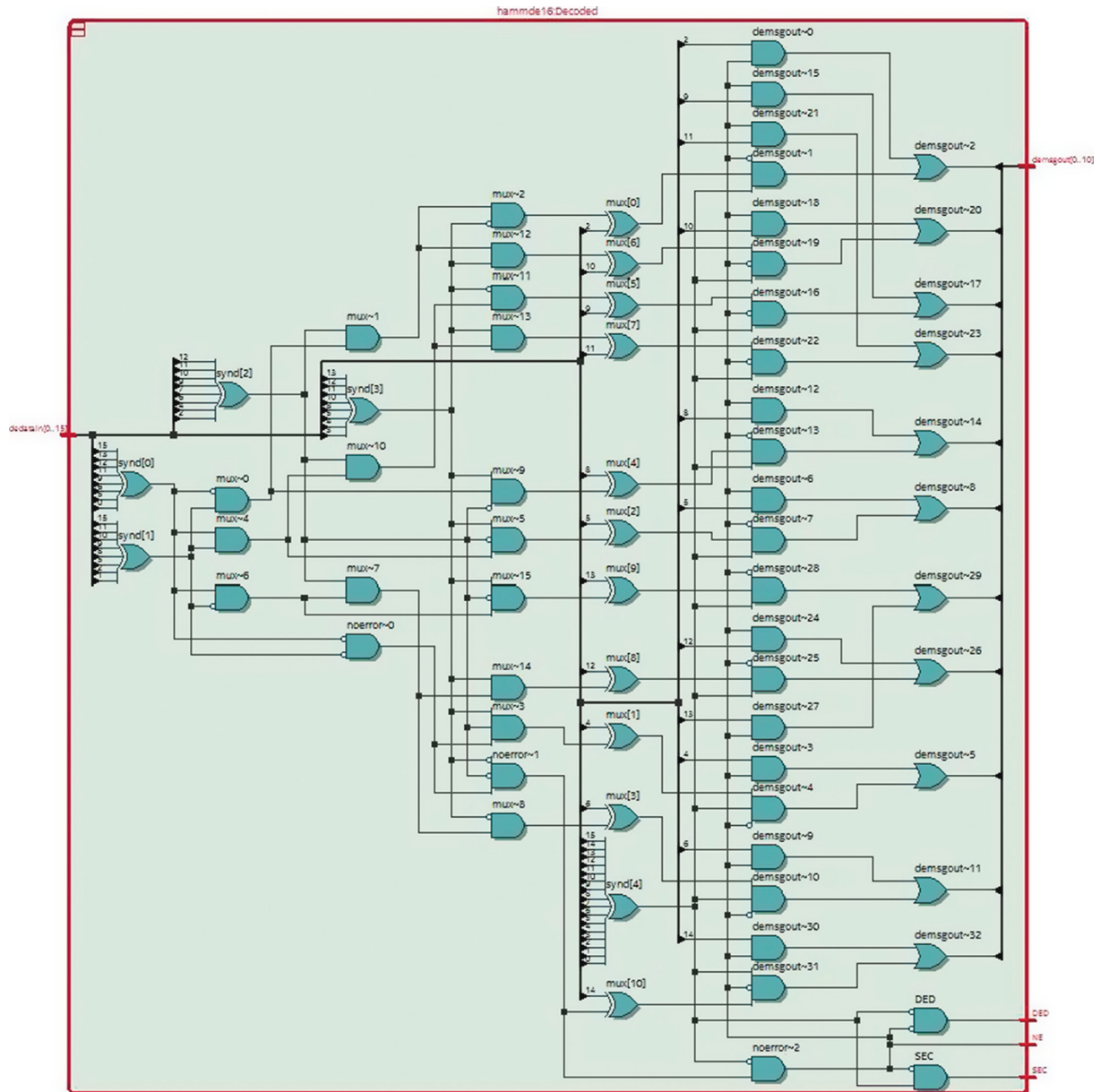
FIGURE 13: RTL overview of the optimized decoder for Hamming [16, 11, 4]_2 .
