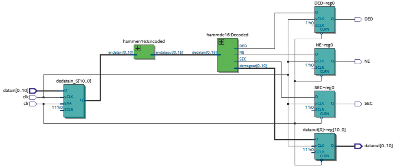
FIGURE 15: Full RTL overview of VHDL code for Hamming [16, 11, 4]_2 .
