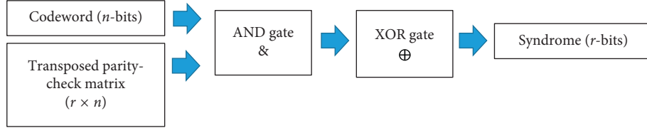
FIGURE 6: Gate/graphical expression of hamming decoder formula.
