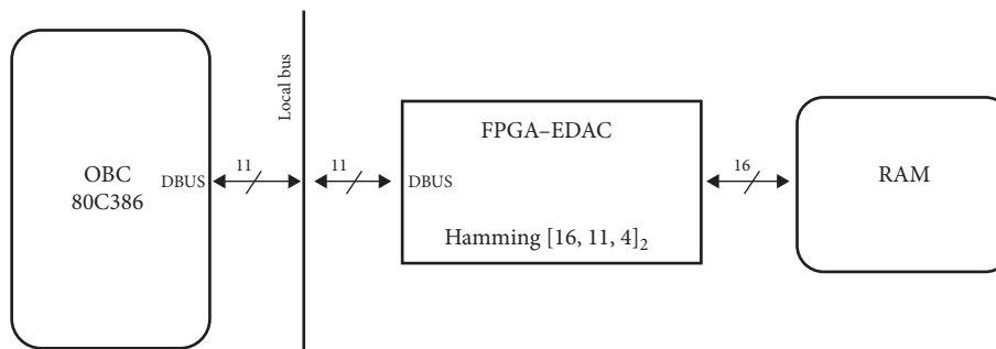
FIGURE 14: Functional block diagram of Hamming [16, 11, 4]_2 .
