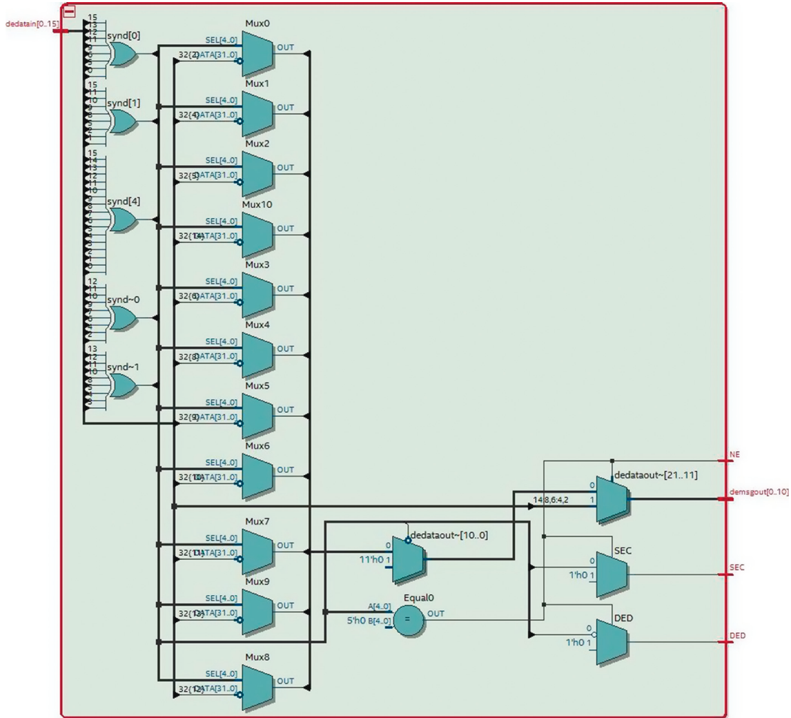
FIGURE 12: RTL overview of the decoder for Hamming [16, 11, 4] 2 .
