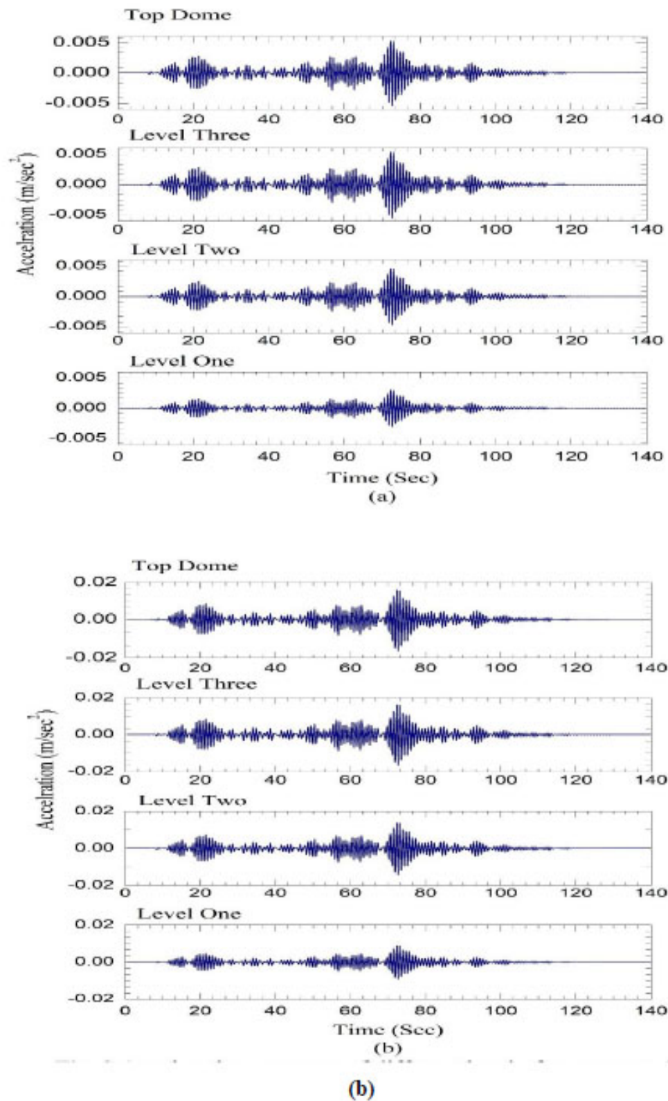
Fig. (9). Acceleration response of different level of monument due to (a) scale input PGA 0.1g (b) scale input PGA 0.3g.
