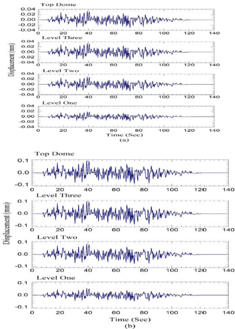
Fig. (10). Displacement response of different level of monument due to (a) scale input PGA 0.1g (b) scale input PGA 0.3g.
