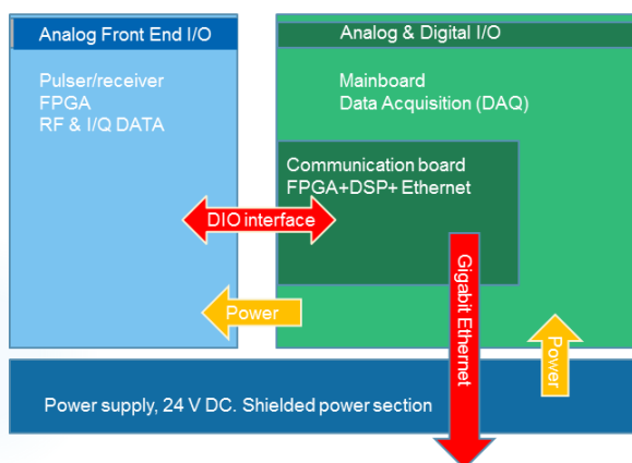
Figure 4: The embedded Flow-Viz TM pulser-receiver, sbRIO and motherboard electronics.
