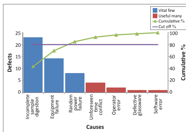
FIGURE 2: Pareto chart – Pareto analysis: Selenium analysis process.
