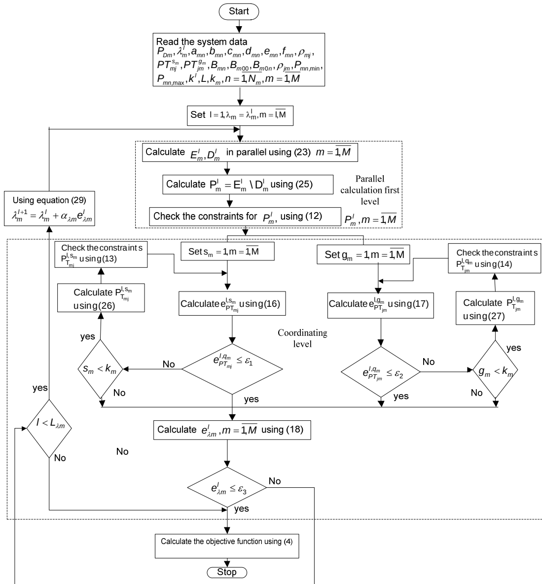
Figure 5. Decomposition-coordinating method flow diagram for parallel solution of the MACEED problem
