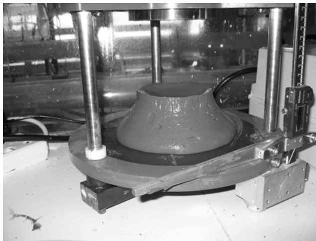
Figure 7. Typical slumped cone formed by kaolinite tailing
