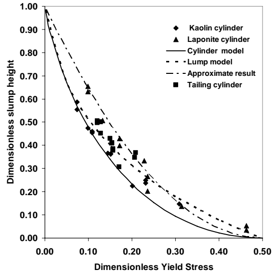
Figure 7. Comparison of different slump models with data
