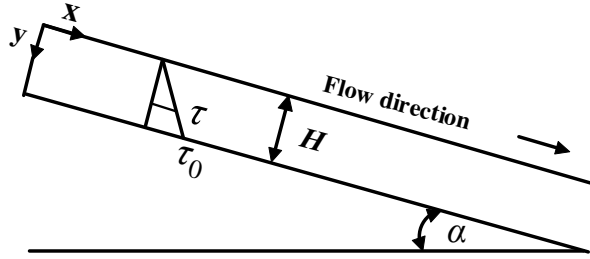
Figure 1: Sheet flow shear stress distribution
