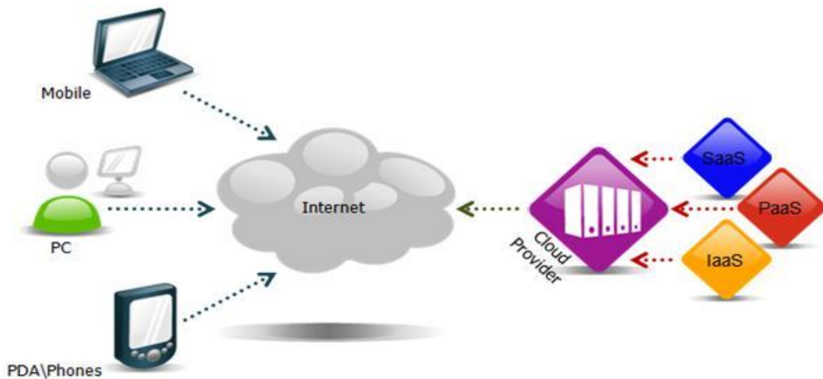
Figure 1. Cloud service
