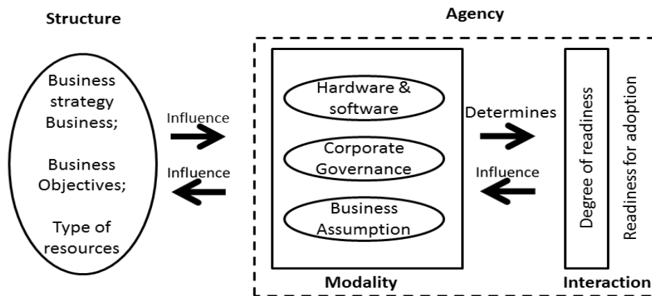
Figure 2. Conceptual framework
