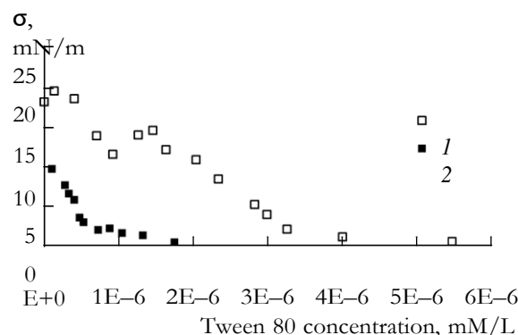
Fig. 4. Interfacial tension dependencies on Tween 80 concentration for PIBSA-Mea/Tween 80 mixtures in the regions below (1) and above (2) the CMC of PIBSA-Mea system.
