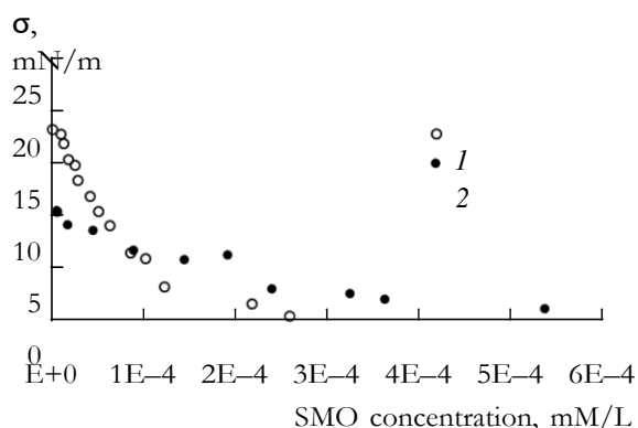
Fig. 3. Interfacial tension dependencies on SMO concentration for PIBSA-Mea/SMO mixtures in the regions below (1) and above (2) the CMC of PIBSA-Mea system.
