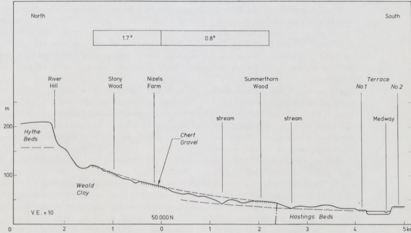
FIGURE 9. Section from River Hill to Summerthorn Wood.
