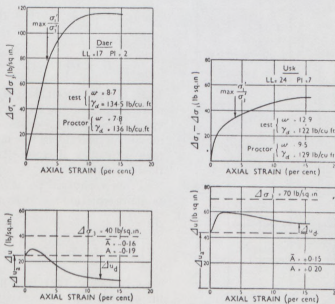
Fig. 3. Undrained triaxial tests on two compacted clay-gravels
