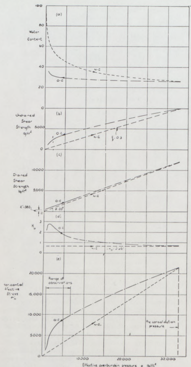
Fig. 4 Geotechnical history of the London Clay at Bradwell Essex.
