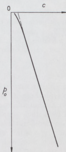
FIG. 4. Relation between undrained shear strength c and effective overburden pressure p_0 for a normally-consolidated clay.
