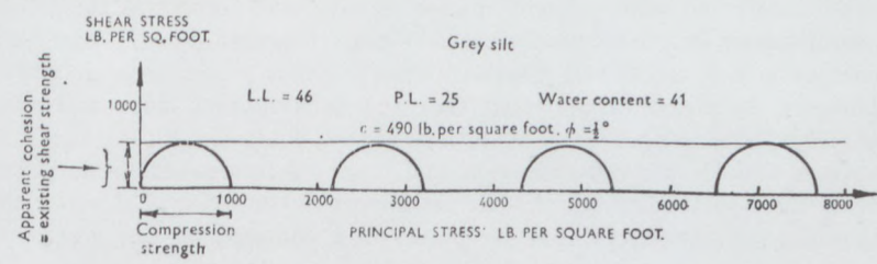
TRIAxIAL TESTS ON GREY SILT, WITH NO CONSOLIDATION PERMITTED UNDER THE APPLIED STRESS.
