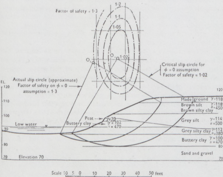
\phi = 0 ANALYSIS OF STABILITY.
