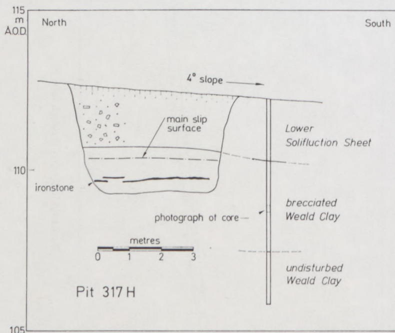
FIGURE 13. Section and borehole at pit 317H 100 m south of lobe E.
