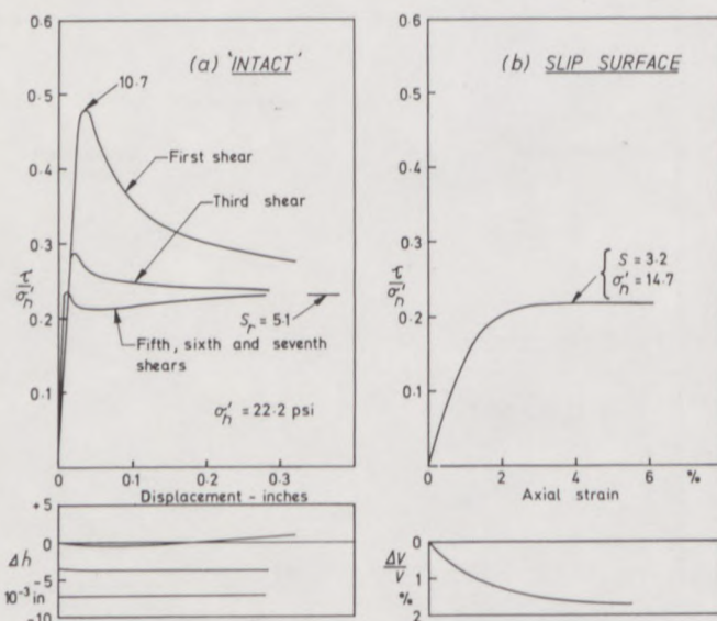
Fig. 6. Walton's Wood; typical stress-displacement curves. Walton's Wood; courbes contrainte-déplacement typiques.
