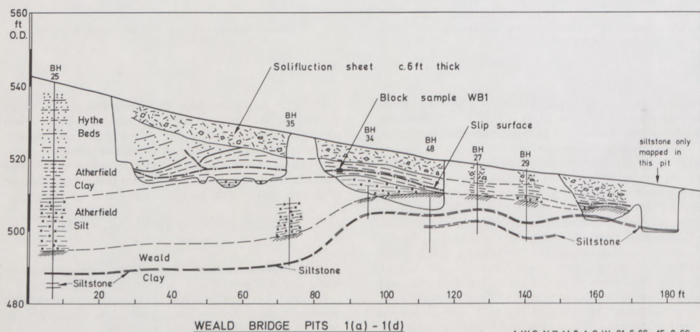
Fig. 13. Sevenoaks: section showing valley bulging and escarpment landslide at Pit WB1.
