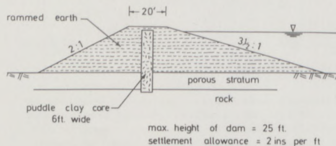
Fig. 2. Earth dam design by John Grundy (1766)
