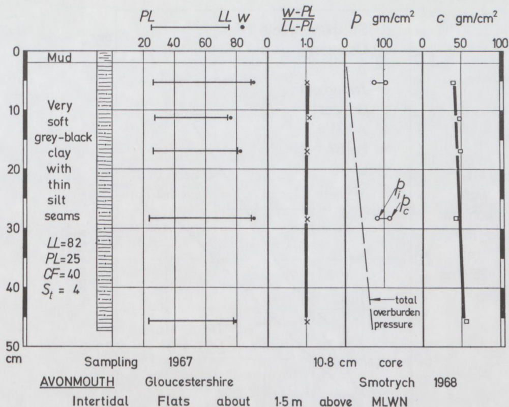
FIG. 10. Intertidal flats at Avonmouth, Gloucestershire. Core taken about 1.5 m above low water mark neap tides (data from Smotrych, op. cit. , 1968).
