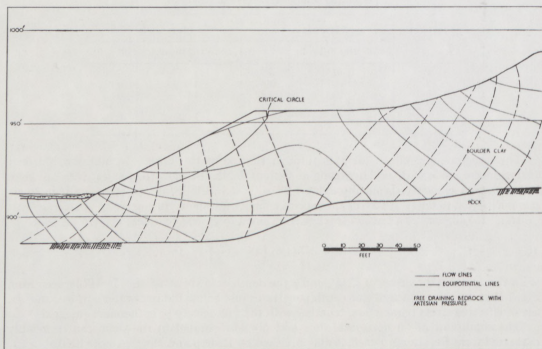
Fig. 5 Flow net B
