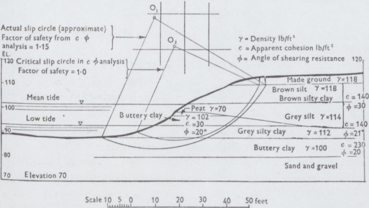
c, φ ANALYSIS OF STABILITY.
