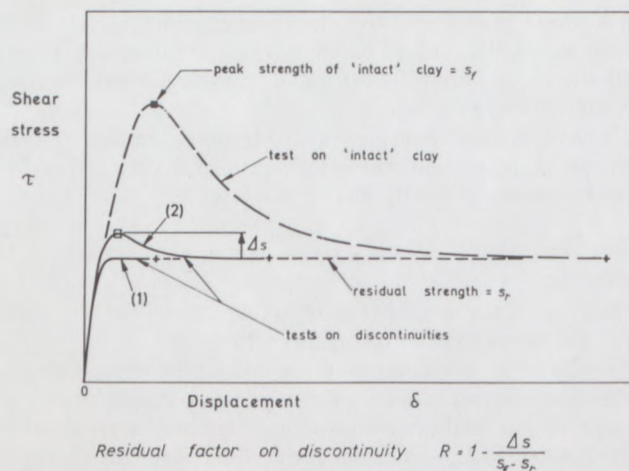
Fig. 2. Stress-displacement curves in tests on a discontinuity and on intact clay.
