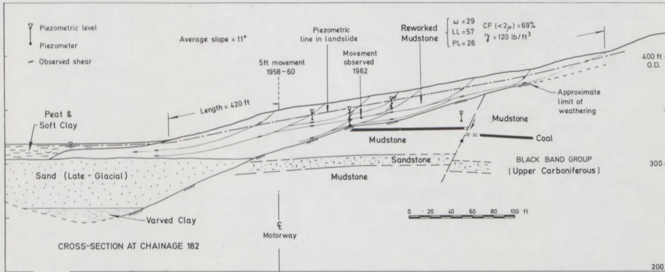
Fig. 3. Geological section through Walton's Wood landslide, Staffordshire.
