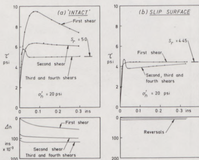
Fig. 10. Guildford; typical stress-displacement curves. Guildford; courbes contrainte-déplacement typiques.
