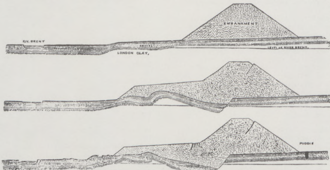
Fig. 10. Brent embankment at Hanwell, Great Western Railway
