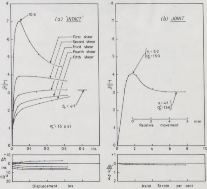
Fig. 32. Wraysbury: typical stress-displacement curves. Blue London clay. Wraysbury: courbes contrainte-déplacement typiques.
