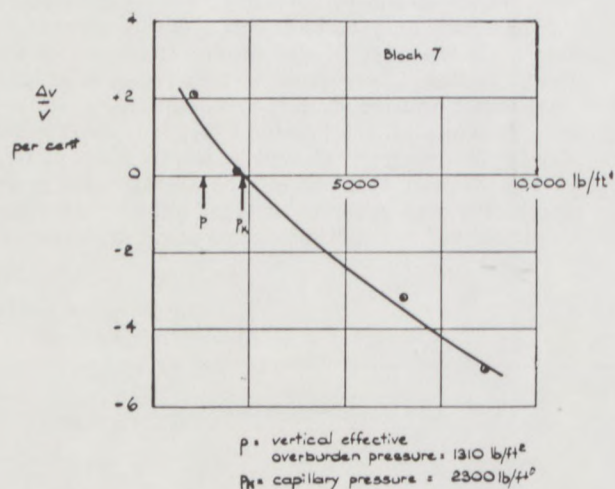
Fig. 5 Swelling pressure test.
