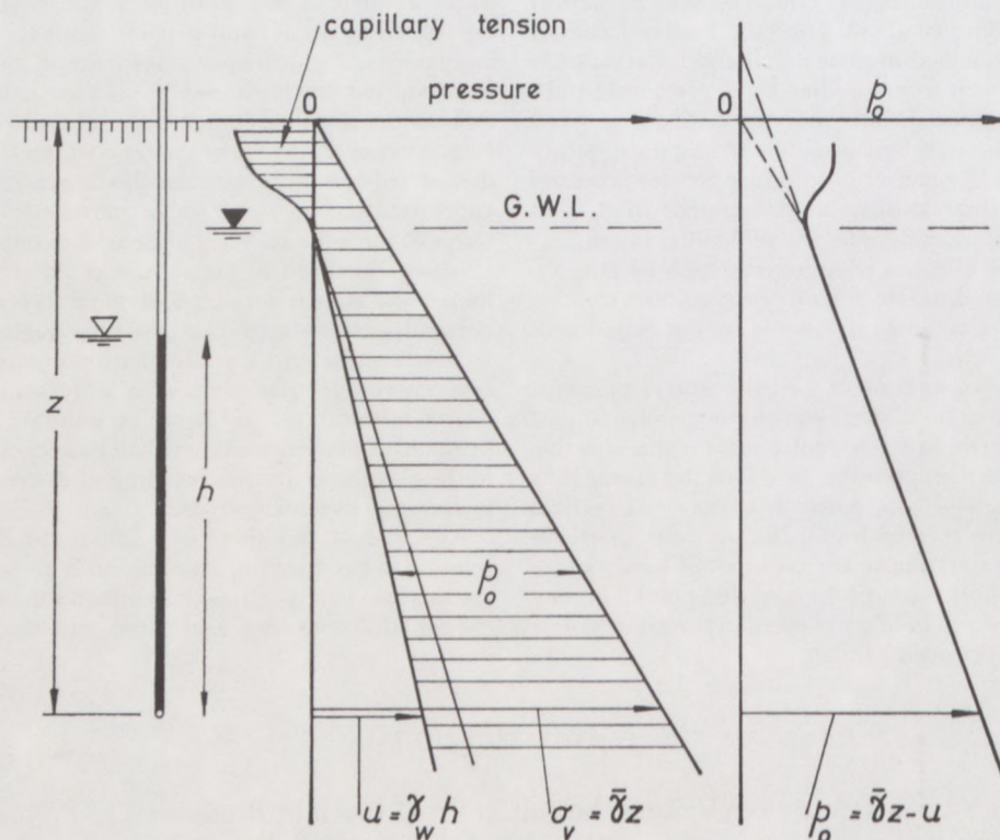
FIG. 1. A typical distribution of total overburden pressure \sigma_v pore pressure u and effective overburden pressure p_o .
