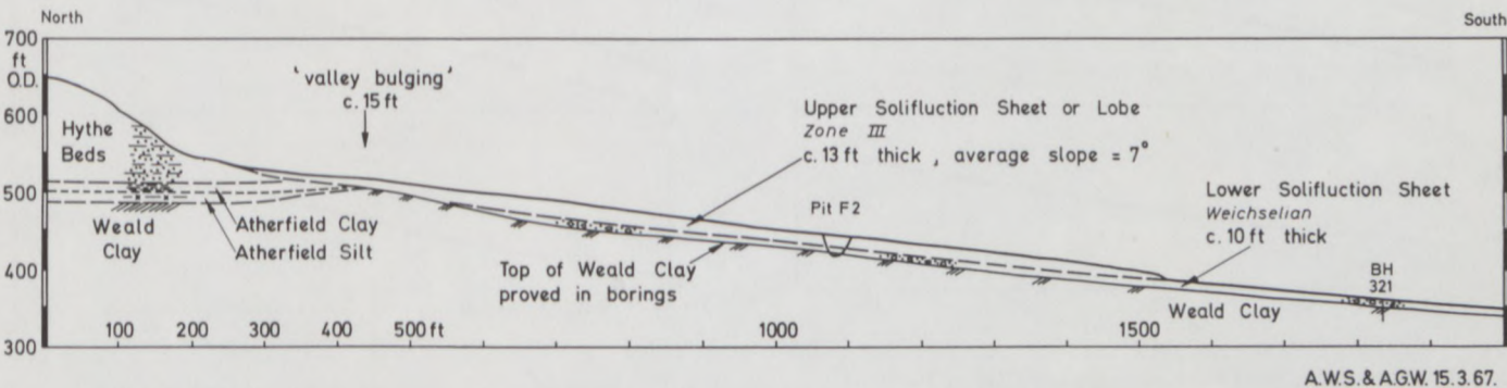
Fig. 12. Geological section of escarpment south of Sevenoaks, Kent. Section through lobe 'F'
