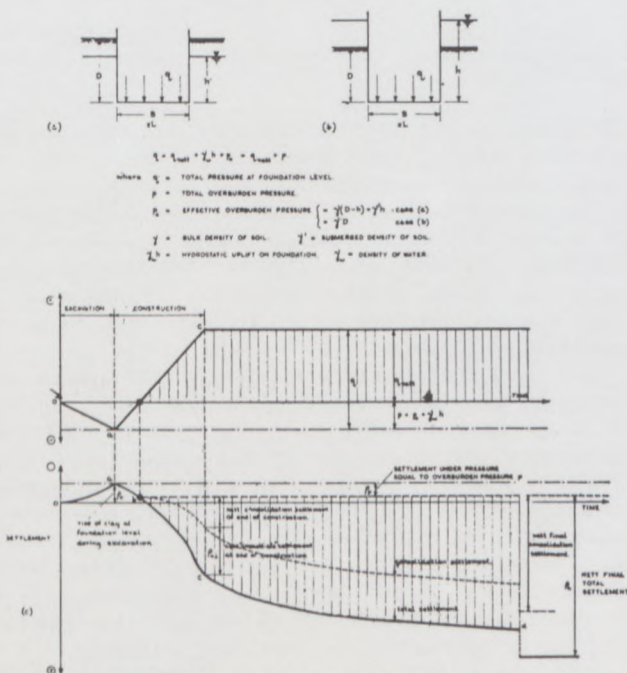
Fig. 1.—Settlement of foundations—General definitions
