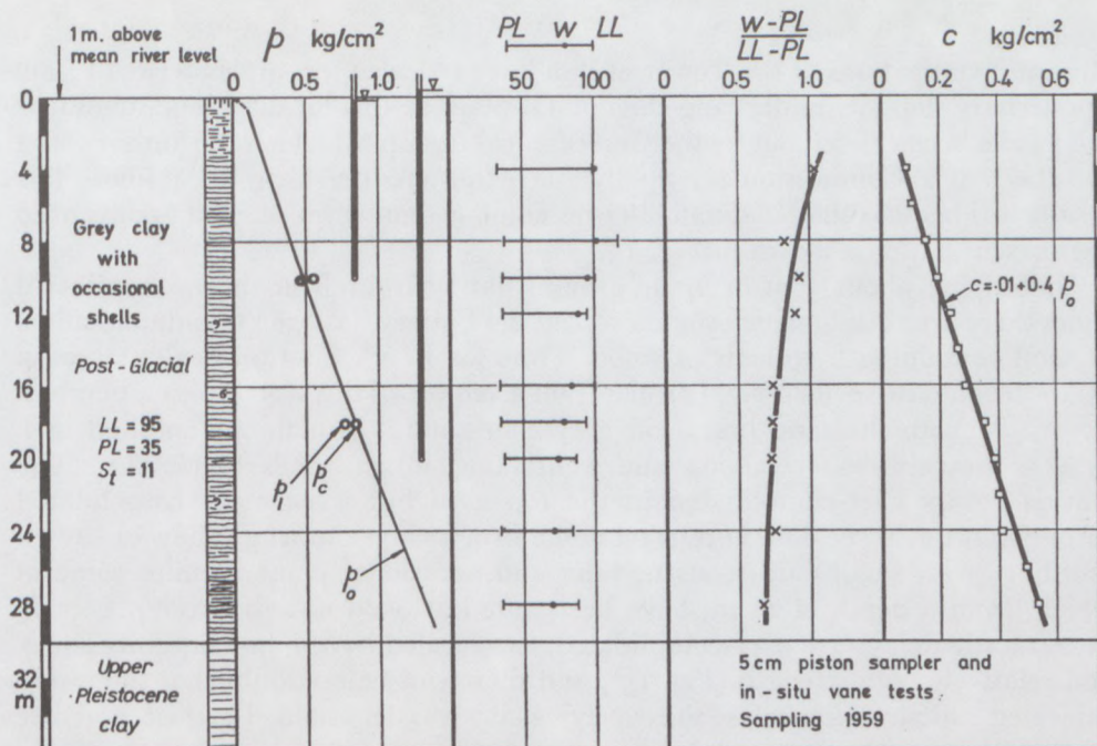
FIG. 14 Borehole No. 15 near the Gota River at Älvängen, Sweden (data from Kallstenius 1963 and in litt. ).
