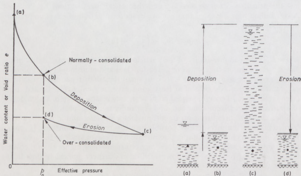
FIG. 2. Normally- and over-consolidated clay.
