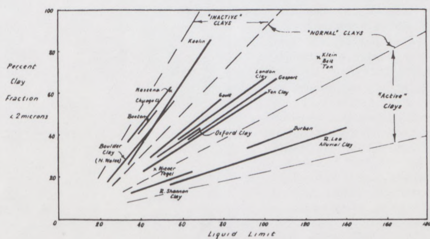
FIG. 2 Relation Between Clay Fraction and Liquid Limit (after Coaling 1966 with extra data)
