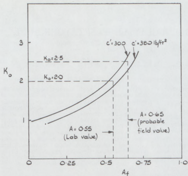
Fig. 7 Relation between K_0 and A_f from the stability analysis of the slip.
