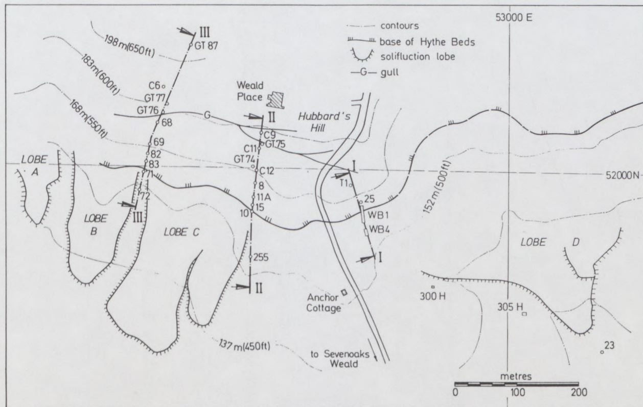
FIGURE 18. Hubbard's Hill: plan.
