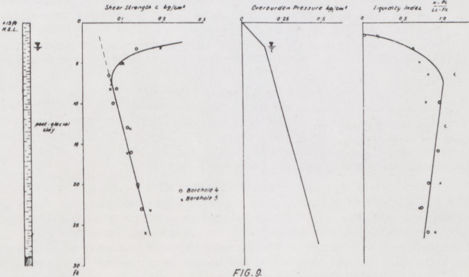
FIG. 9. Properties of a Post-glacial Clay near Lake Hälsjön, Sweden (data reproduced by permission from private communication from R. Kjellman)
