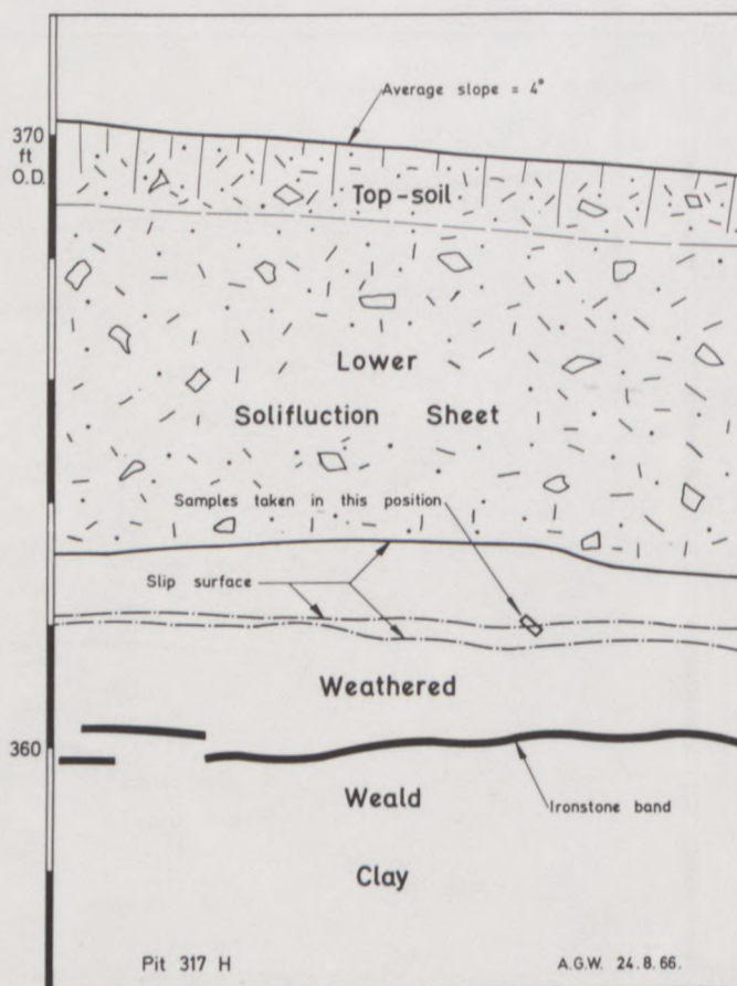
Fig. 20. Sevenoaks: section through lower solifluction sheet at Pit 317H. Sevenoaks: coupe de la nappe inférieure de solifluction à la fouille 317H.
