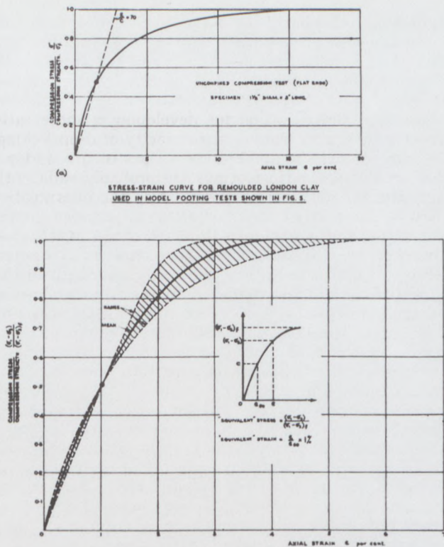
Fig. 6. "Equivalent" stress strain curves for undisturbed clays ( E/c = 100 ) As before, equation (8) is more conveniently written in the form \epsilon = \frac{\sigma_1 - \sigma_3}{(\sigma_1 - \sigma_3)_t} \cdot \frac{(\sigma_1 - \sigma_3)_t}{c} \cdot \frac{I}{E/c} \dots \dots (9) In saturated clays with no water content change under applied stress \frac{(\sigma_1 - \sigma_3)_t}{c} = 2.0 . Thus
