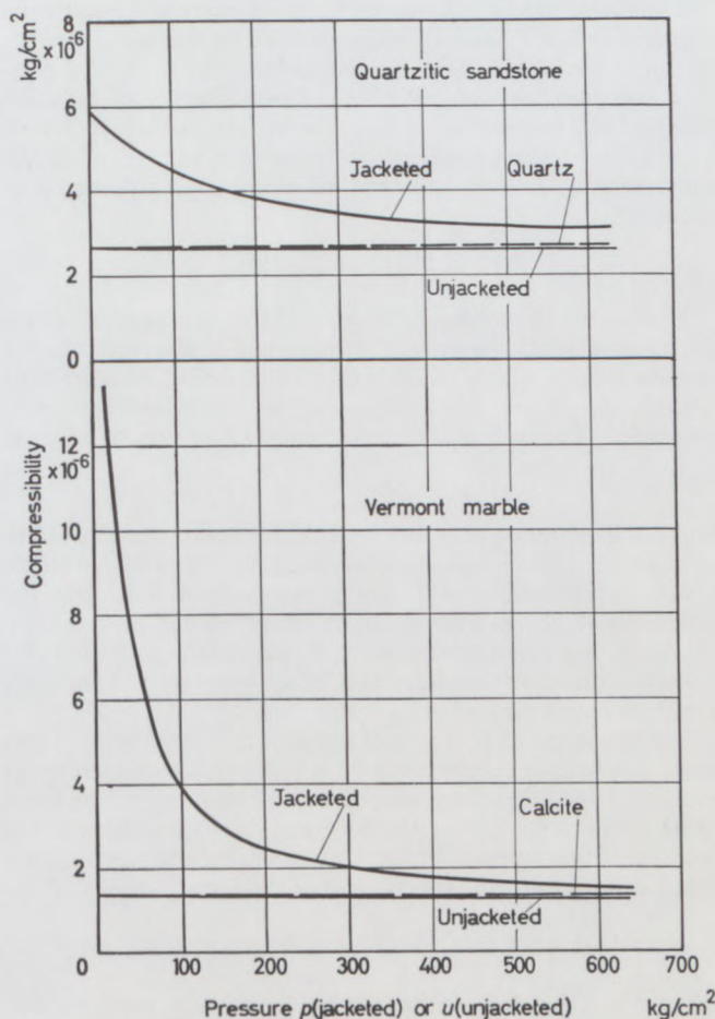
Fig. 8 Compressibility tests (ZISMAN, 1933 and BRIDGMAN, 1928)
