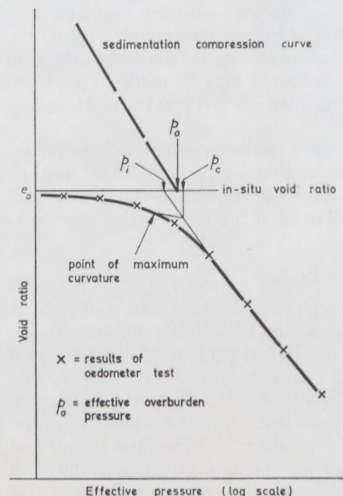
FIG. 3. Typical results of an oedometer test on normally-consolidated clay.
