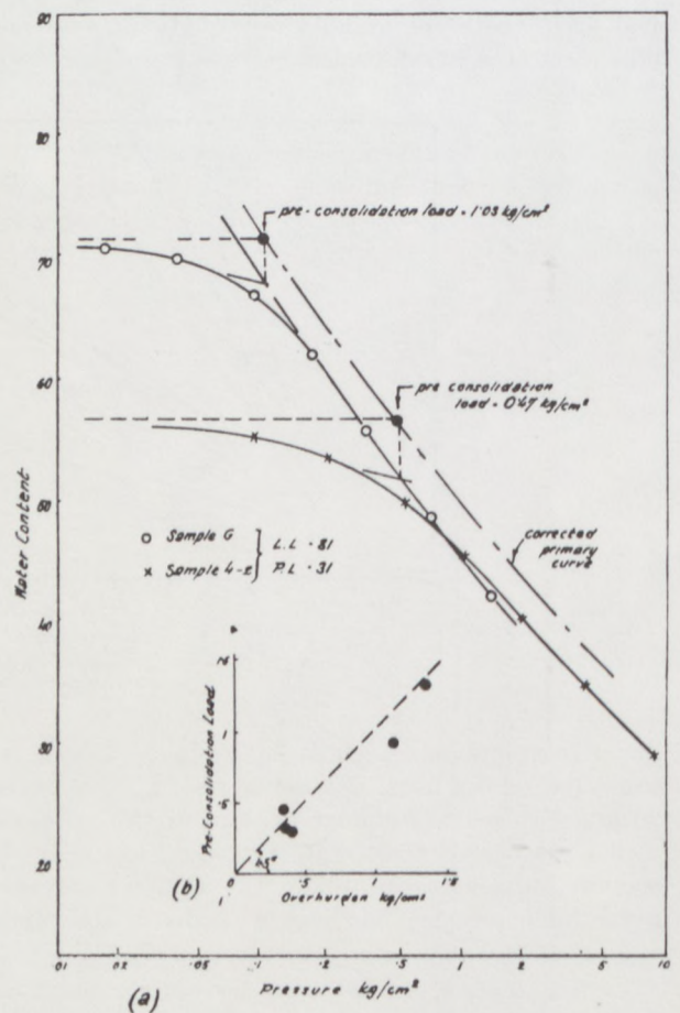
FIG. 4. Consolidation Test Results on Gosport Post Glacial Clay (Skempton 1948a)
