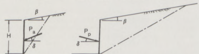
\delta and \beta shown + ve
