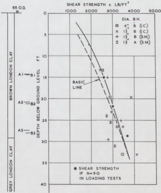
Fig. 4. Shear strengths at site of Kensal Green loading tests (1951)
