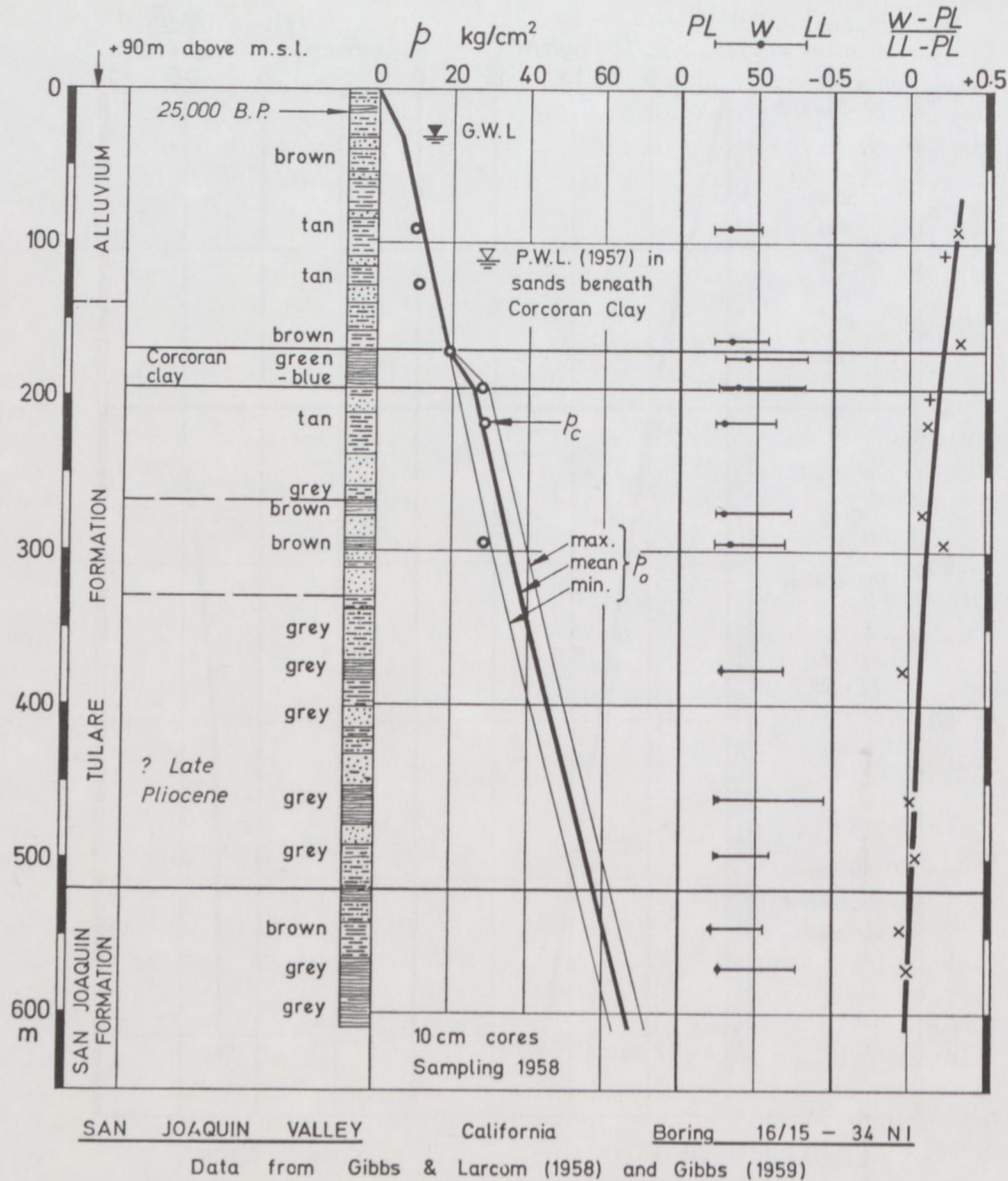
FIG. 17. Boring 16/15-34 NI near Cantua Creek in San Joaquin Valley, California (data from Gibbs & Larcom 1958; Gibbs 1959).
