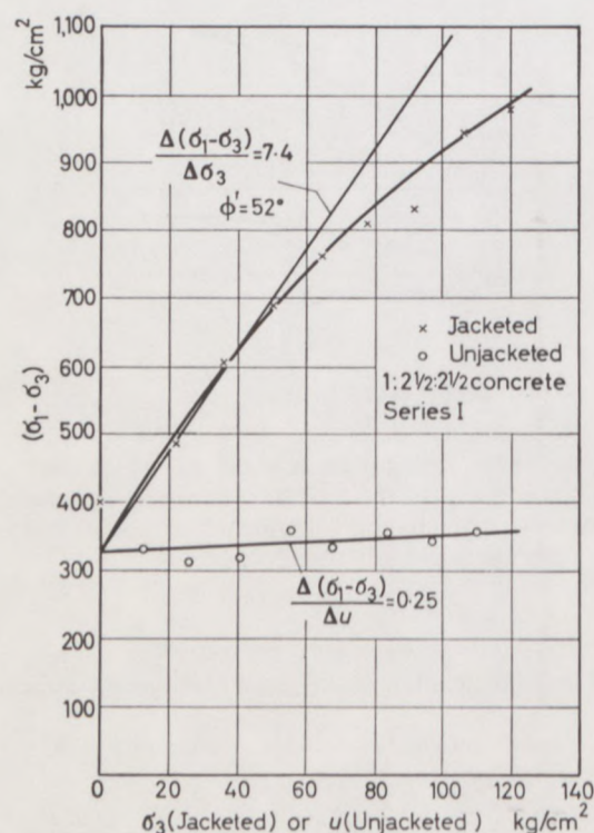
Fig. 7 Triaxial tests on concrete (McHENRY, 1948)
