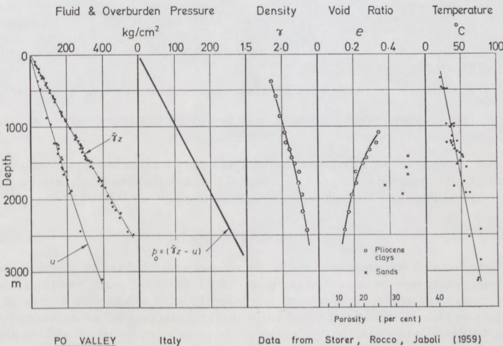
FIG. 20. Summary of results from borings in the Po Valley (data from Storer 1959, Rocco & Jaboli 1958).
