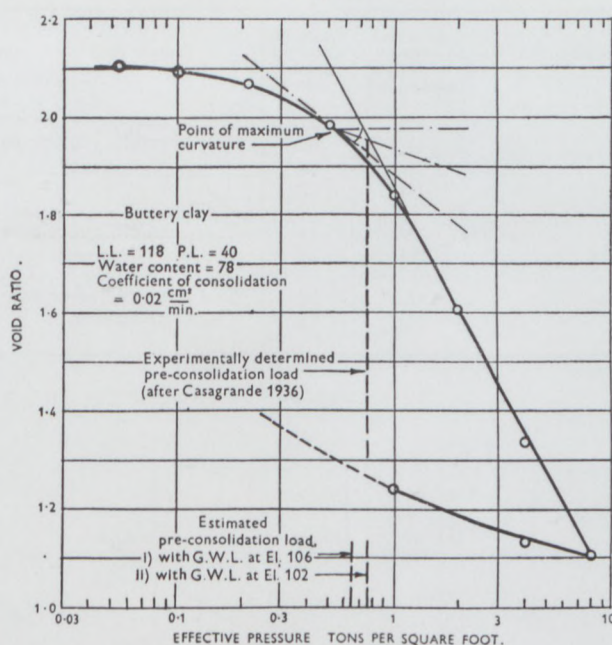
PRE-CONSOLIDATION LOAD OF BUTTERY CLAY AT ELEVATION 83.
