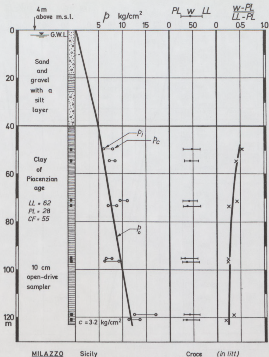
FIG. 16. Boring at Milazzo, Sicily (Croce in litt.).
