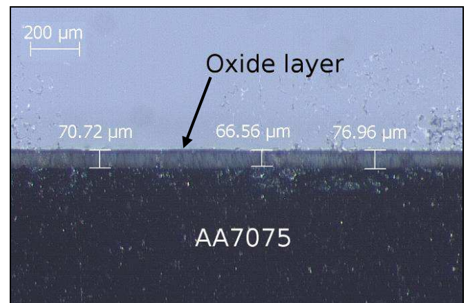
Figure 2: The hard anodised layer (aluminium oxide) has an average thickness of 70 \mu\text{m} .
