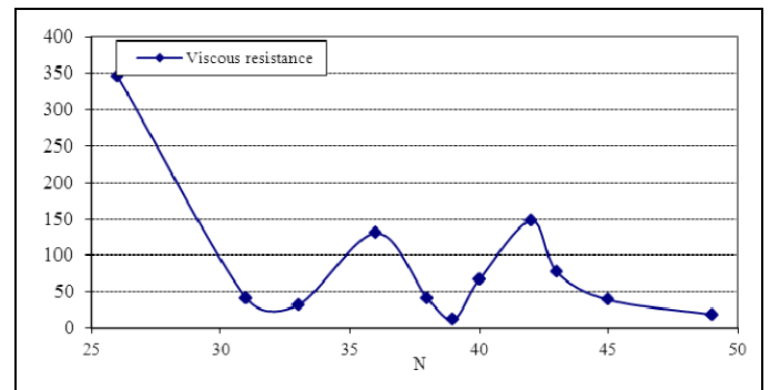
Fig.4. Acoustic power, viscous resistance plotted as a function of N
