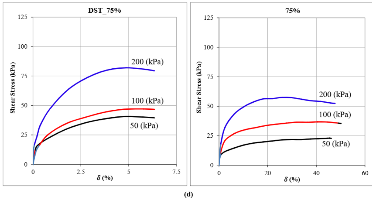
Figure 7 (a-d). 10%, 25%, 50% and 75% kaolinite clay stress-strain curves for DST and DSST test results
