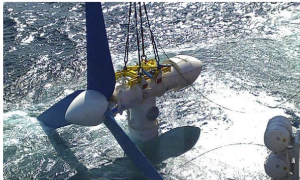
Figure 27. AR1000 tidal stream turbine (© Simec Atlantis Energy) [20].
