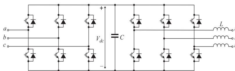
Figure 9. Back-to-back converter.
